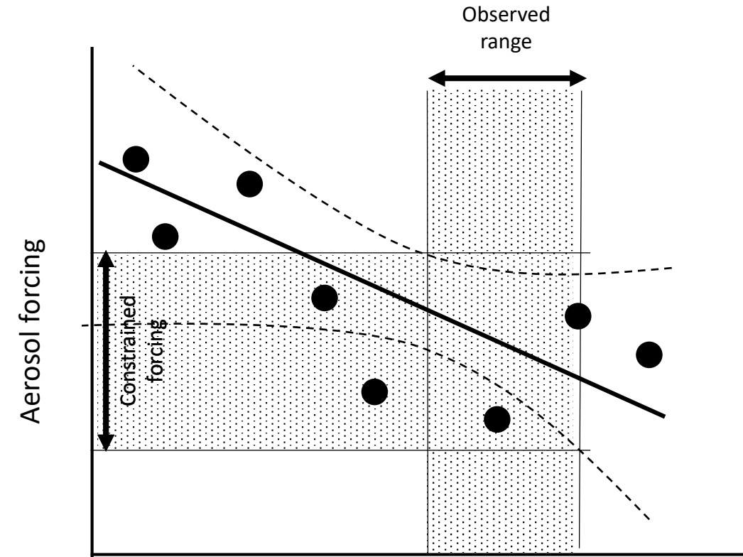
(a) Change in surface radiation
