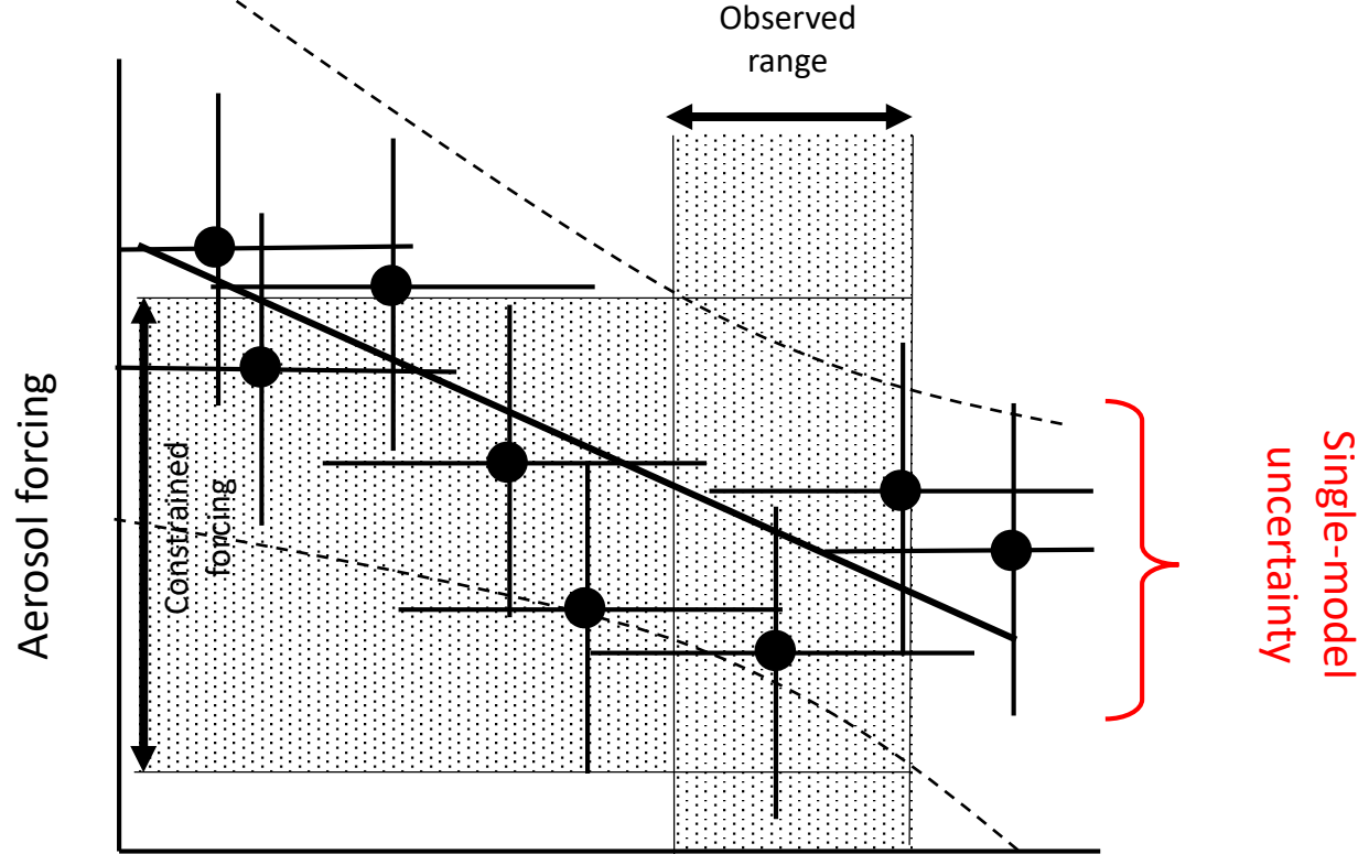
(b) Change in surface radiation
