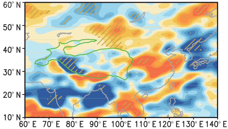
(b) Surface precipitation
