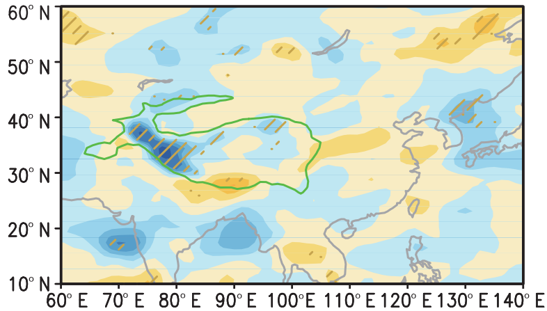
(a) 500 hPa omega
