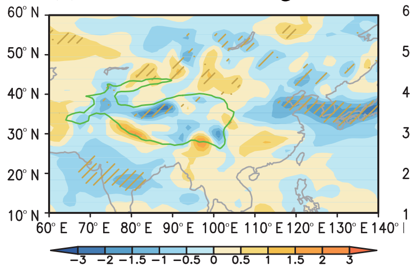
(c) 500 hPa Omega
