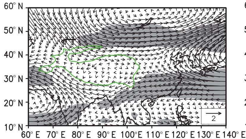
(a) 500 hPa wind field
