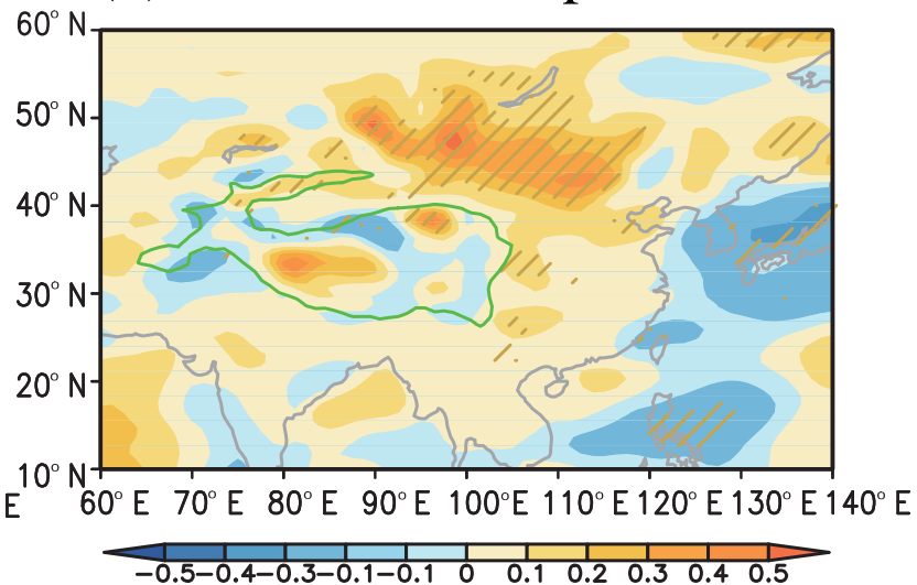
(b) 10 m wind speed
