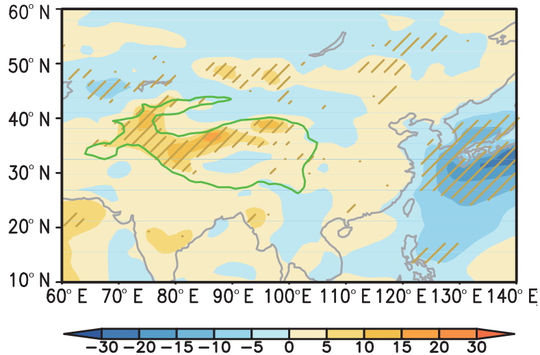
(b) Latent heat flux
