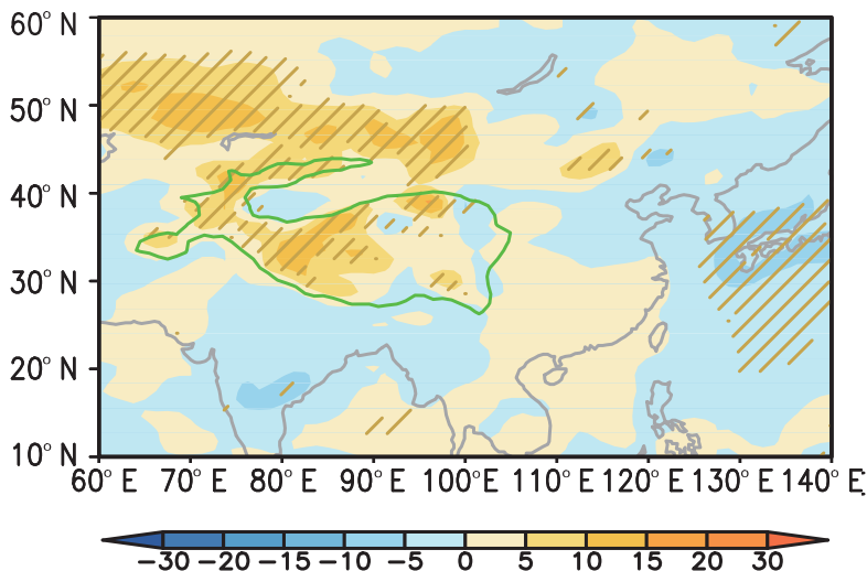
(c) Sensible heat flux
