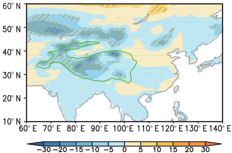
(a) Snow cover fraction
