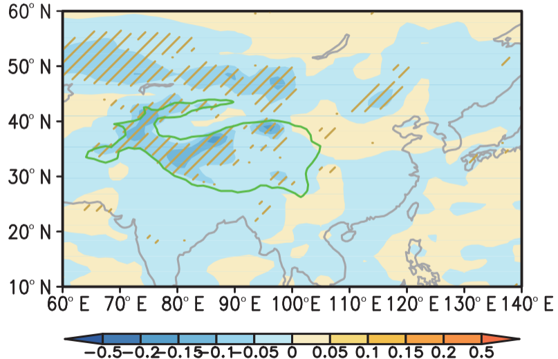
(b) Diff. in broadband surface albedo
