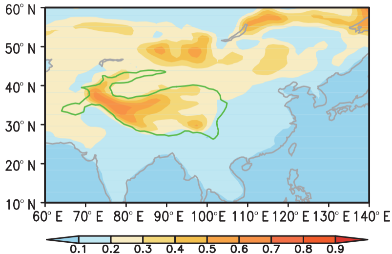
(a) Broadband surface albedo
