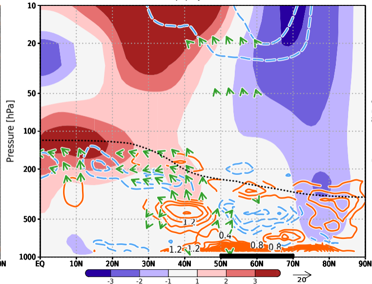
(b) QBO-W
