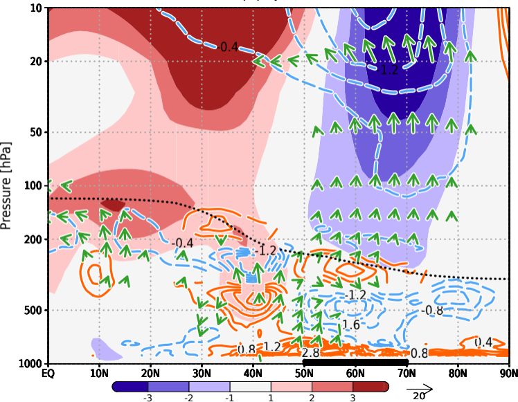
(a) QBO-E
