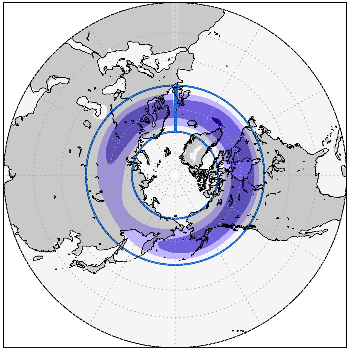
(b) Deviation of WAFz100 (WN2) (16NOV-30NOV)
