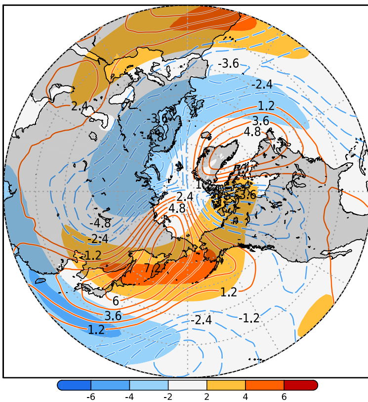
(a) Climatological V' , T'_{100} (01NOV-15NOV)
