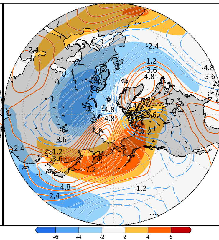
(b) Climatological V' , T'_{100} (16NOV-30NOV)
