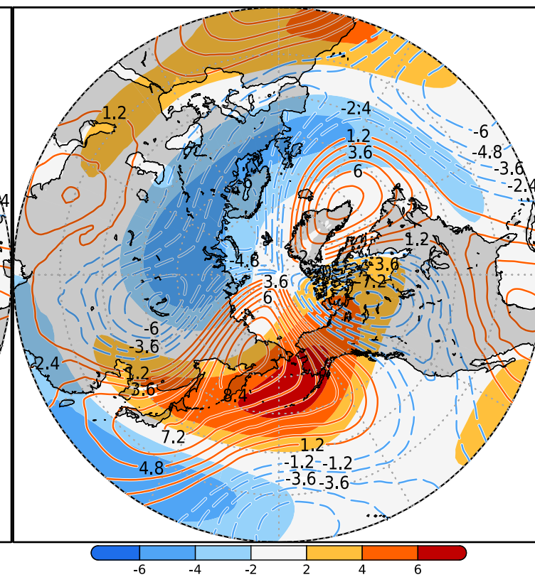
(c) Climatological V' , T'_{100} (01DEC-15DEC)
