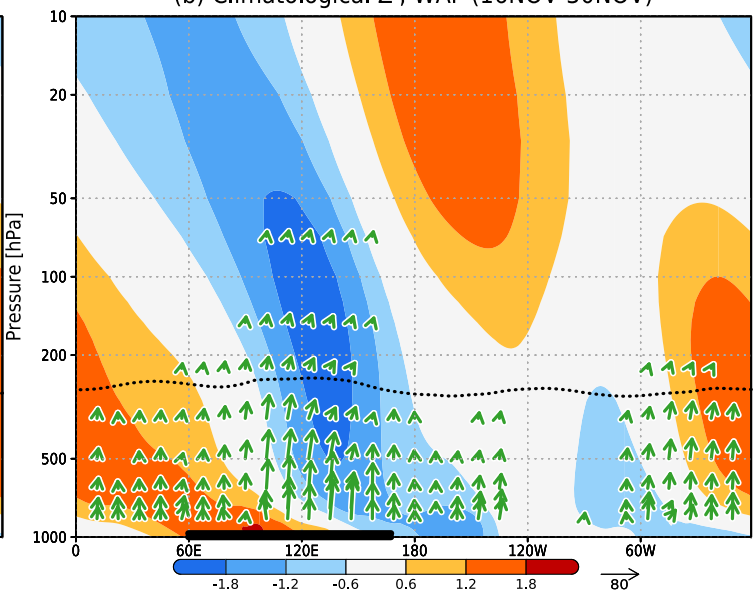
(b) Climatological Z' , WAF (16NOV-30NOV)
