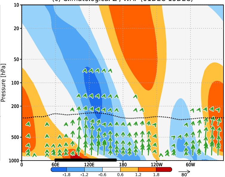
(c) Climatological Z' , WAF (01DEC-15DEC)
