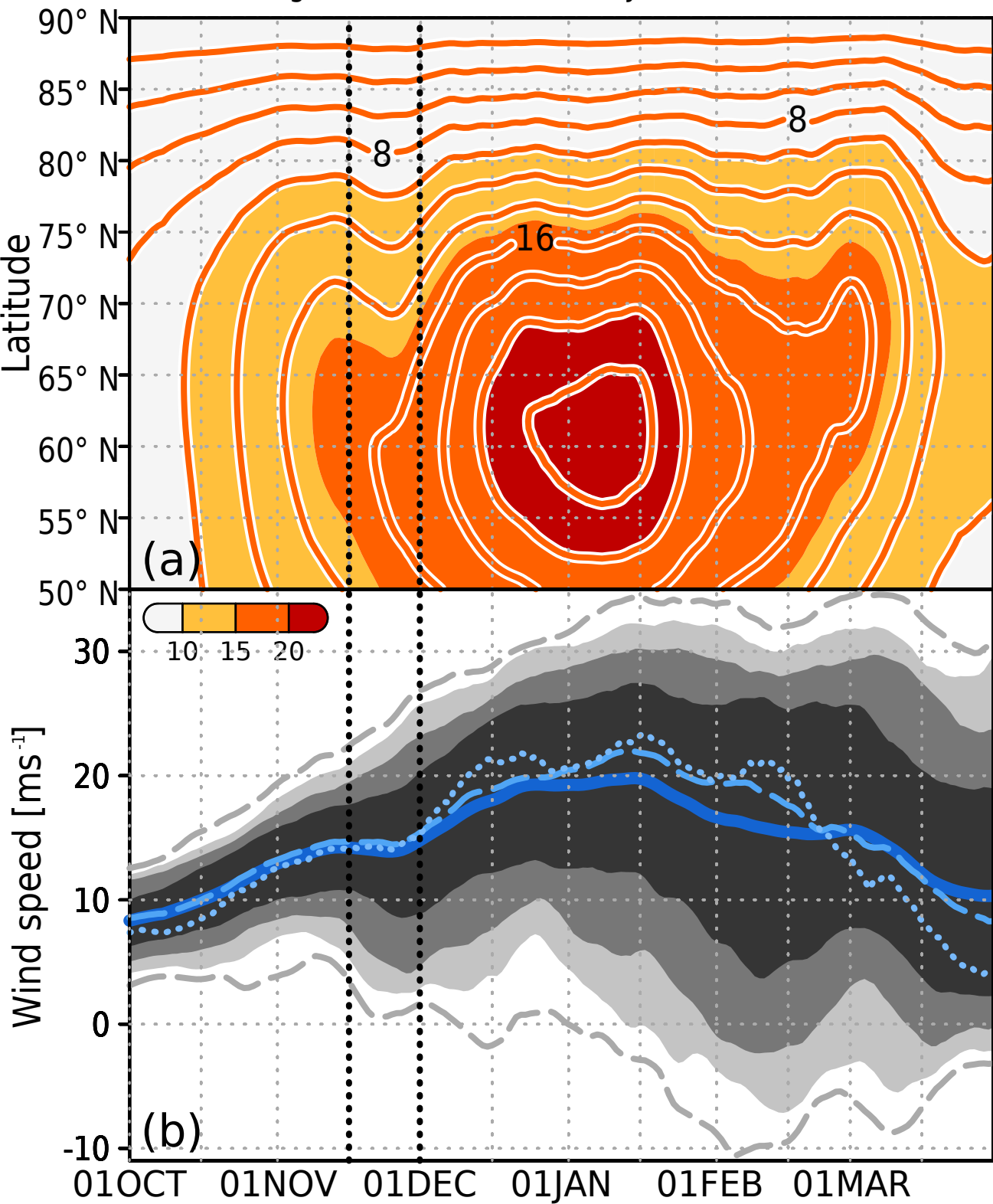
Climatological zonal-mean U50, PNJ index (50 hPa, 60-80° N)
