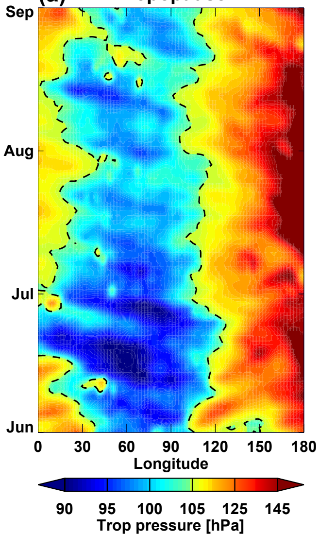
(a) Tropopause
