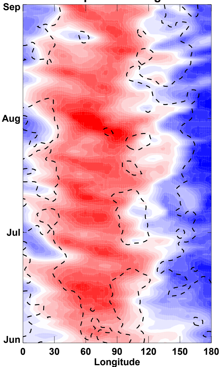
Geopotential height
