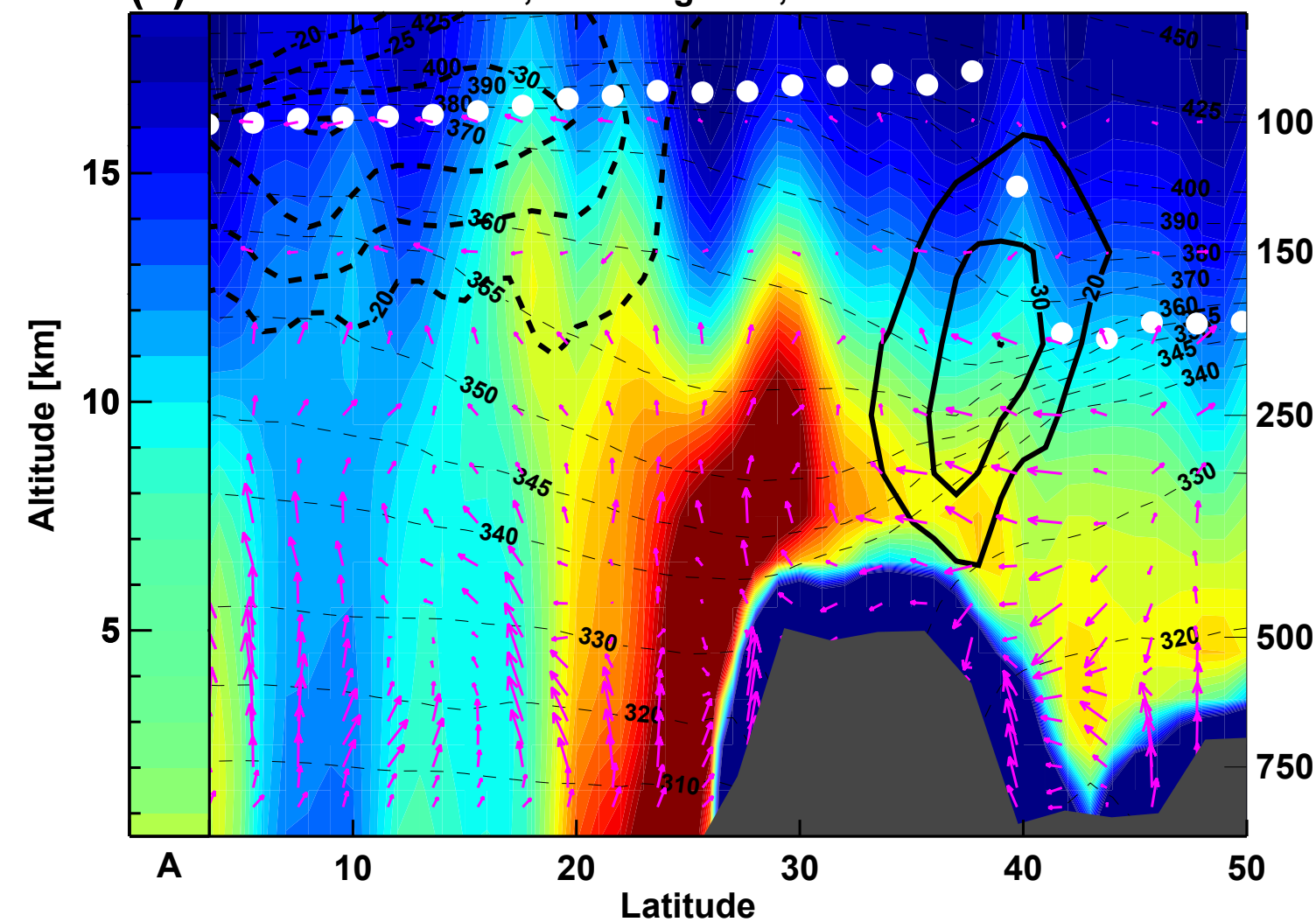
(c) IASI CO, 50.0 longitude, 2008/07/22
