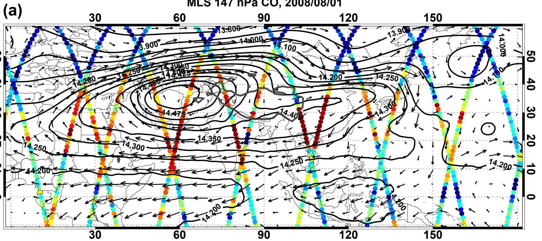
MLS 147 hPa CO, 2008/08/01
