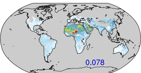
(c) JJA
