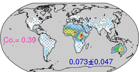
(g) JJA
