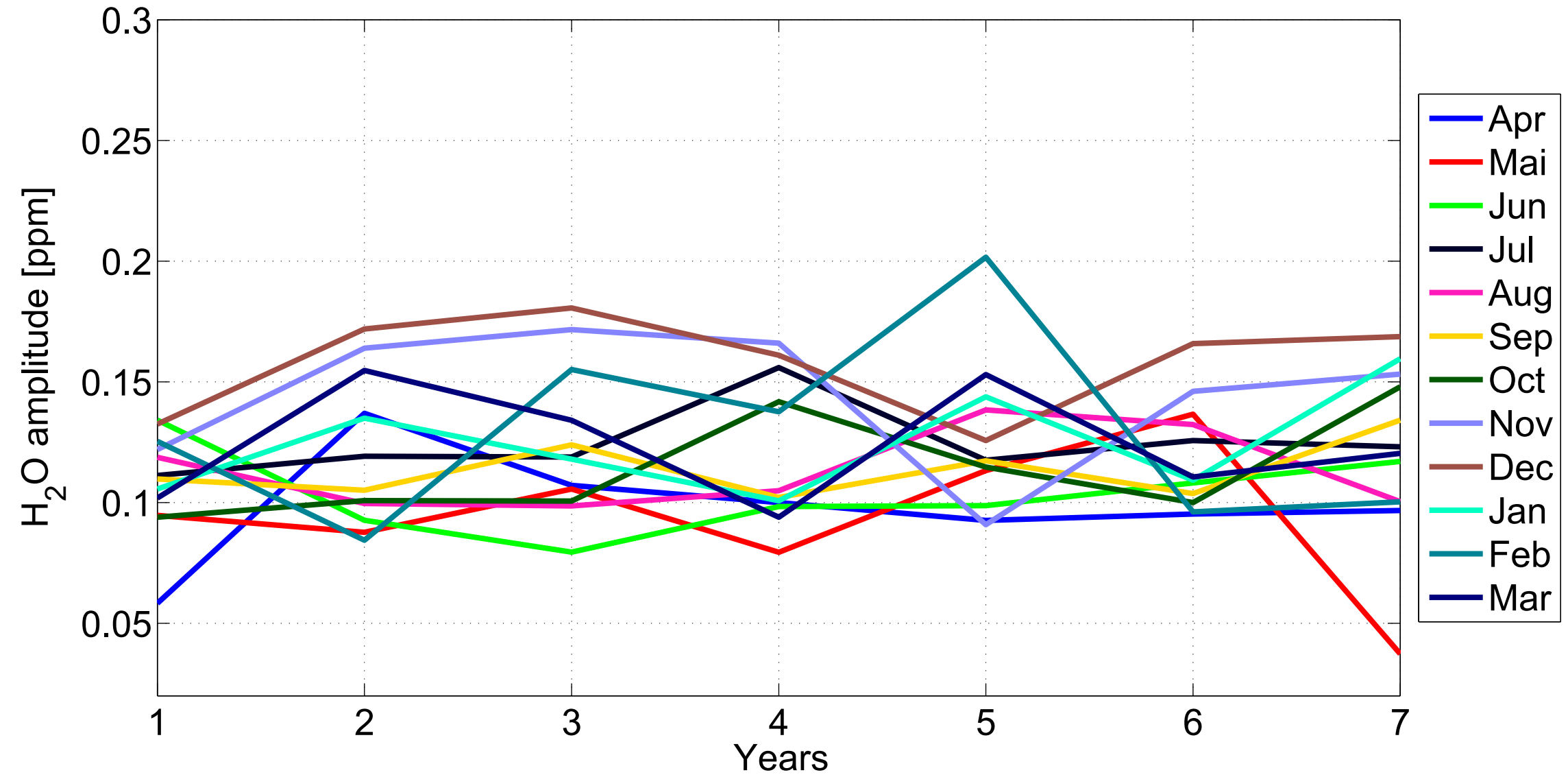
(b) Q2DW (43–53 h) amplitude evolution averaged between 0.2 and 1 hPa
