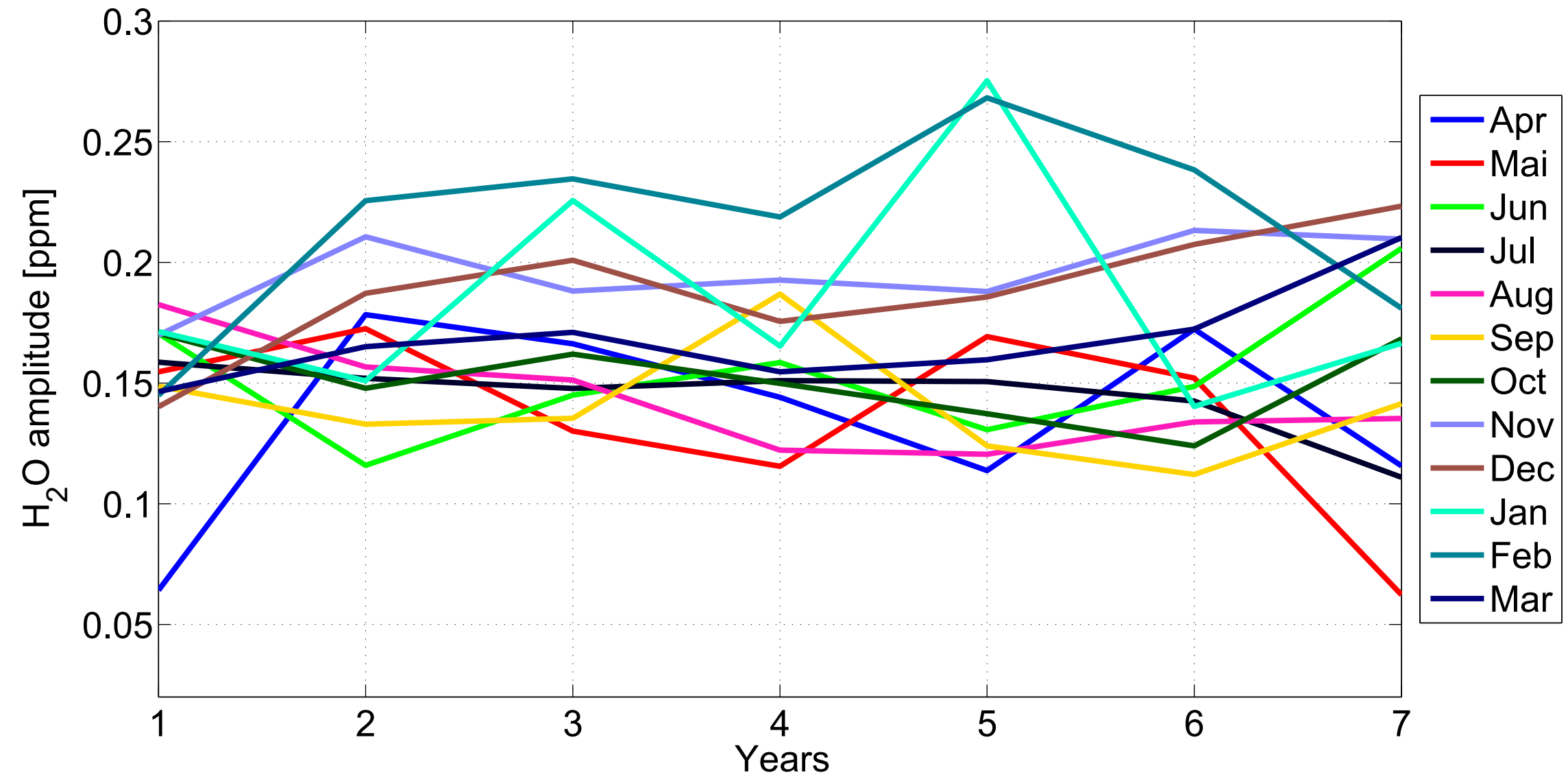
(a) Q2DW (43–53 h) amplitude evolution averaged between 0.05 and 0.2 hPa
