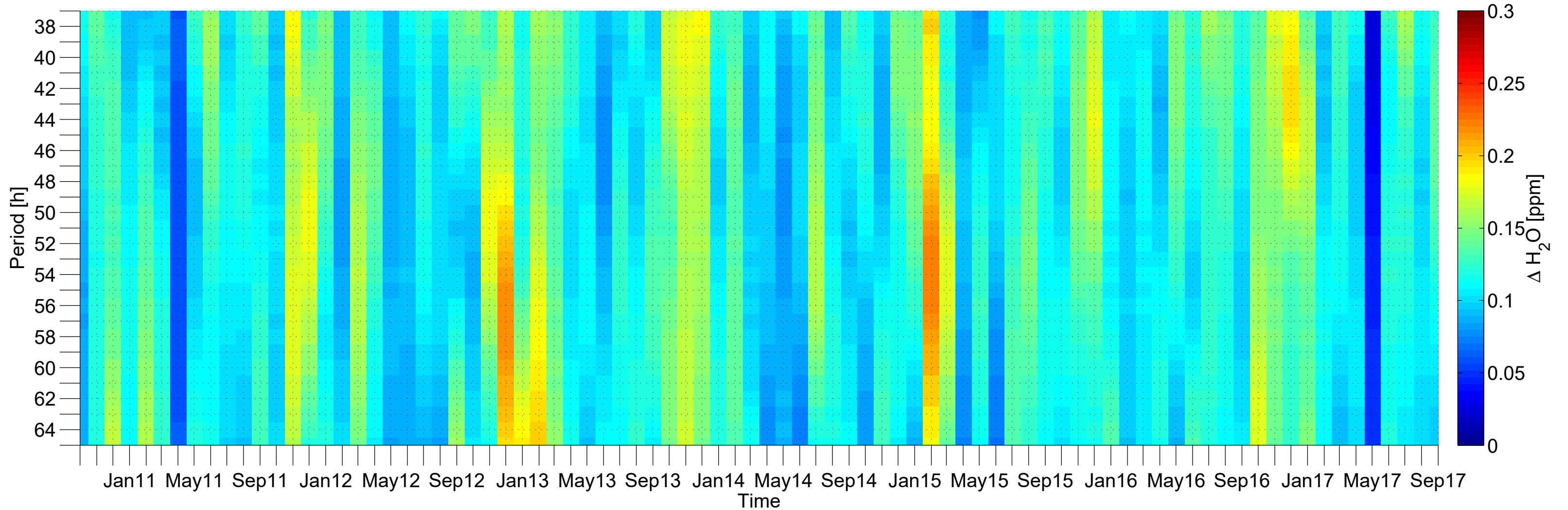
(b) Q2DW amplitude versus period evolution averaged between 0.2 and 1 hPa
