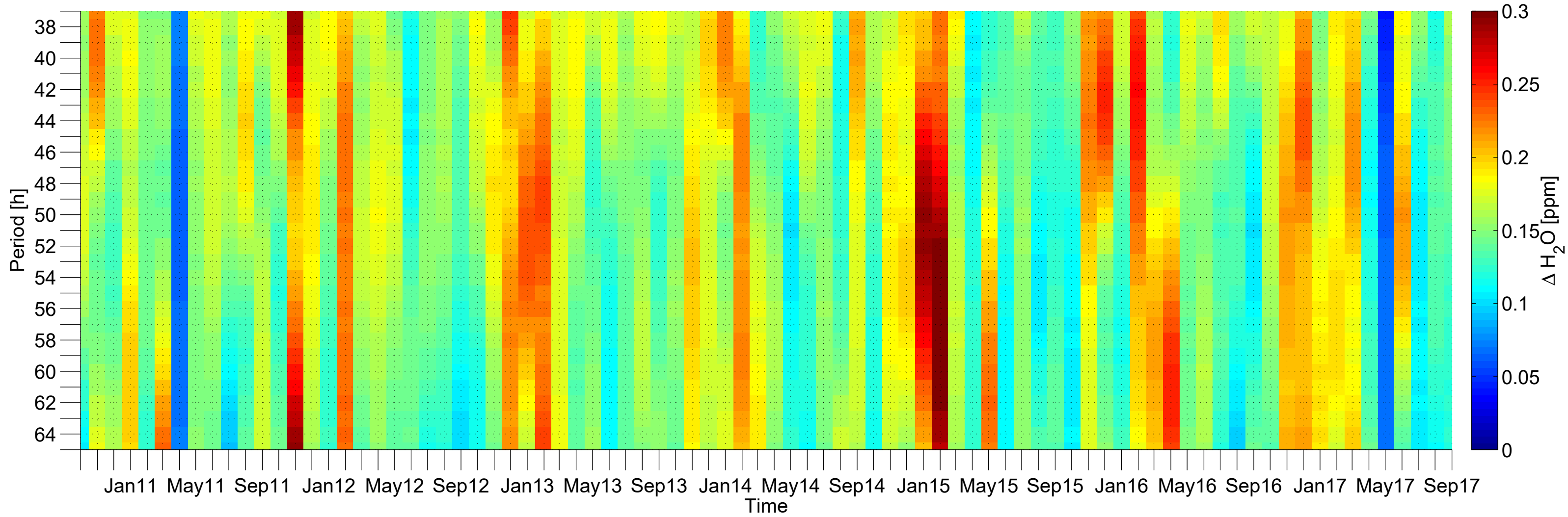
(a) Q2DW amplitude versus period evolution averaged between 0.05 and 0.2 hPa
