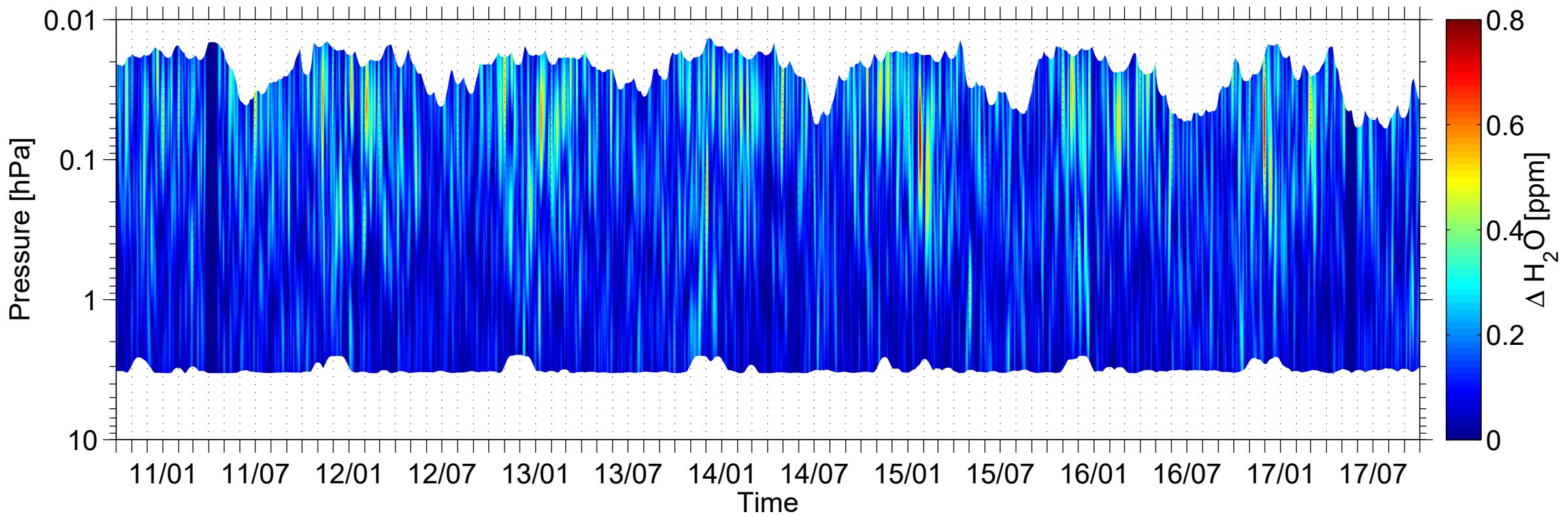
(a) Q2DW (43h – 53h) absolute amplitude in H 2 O tracer
