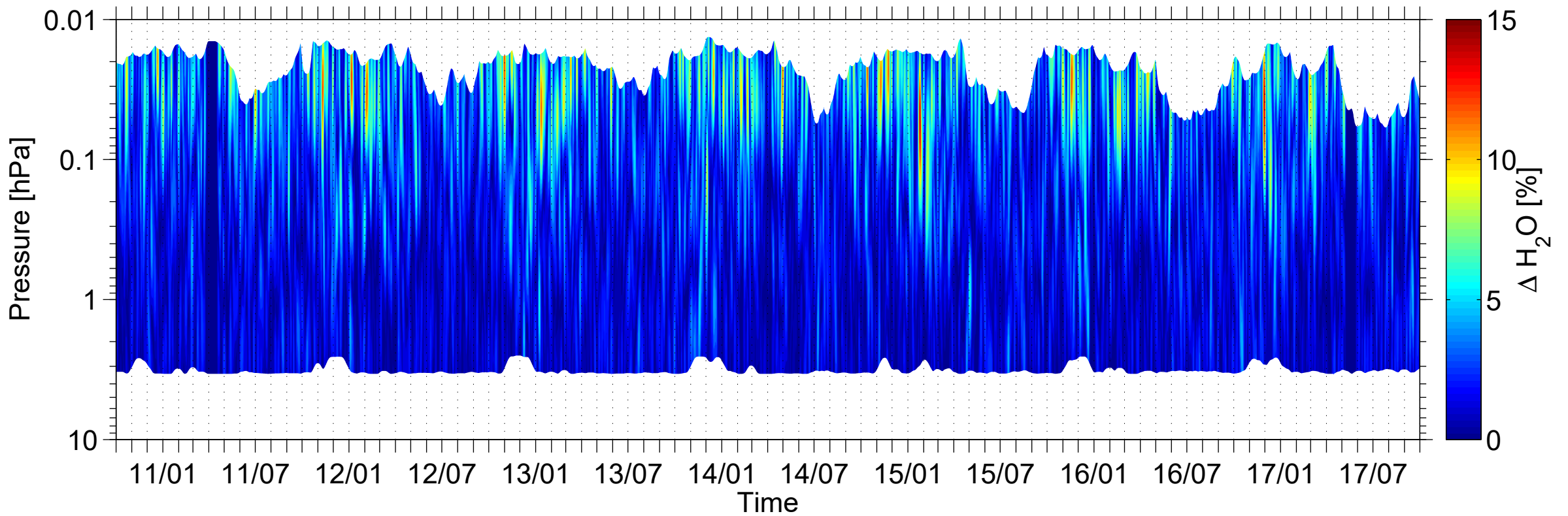
(b) Q2DW (43h – 53h) relative amplitude in H 2 O tracer
