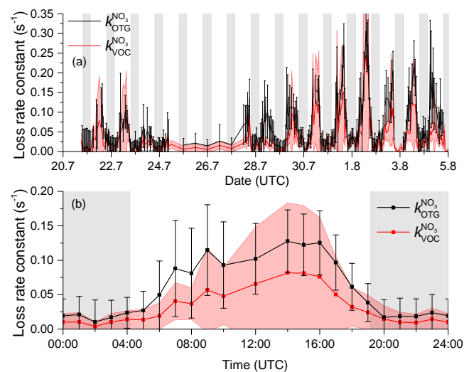
Figure 5. (a) Time series of k_{\text{VOC}}^{\text{NO}_3} and k_{\text{OTG}}^{\text{NO}_3} . The error bars on the k_{\text{OTG}}^{\text{NO}_3} measurements are total uncertainty calculated as described by Liebmann et al. (2017). The uncertainty in k_{\text{VOC}}^{\text{NO}_3} (shaded red area) is dominated by uncertainty in the mixing ratios of the VOCs. Panel (b) is a campaign-averaged diel profile of the same parameters, whereby the uncertainties also include variability.
