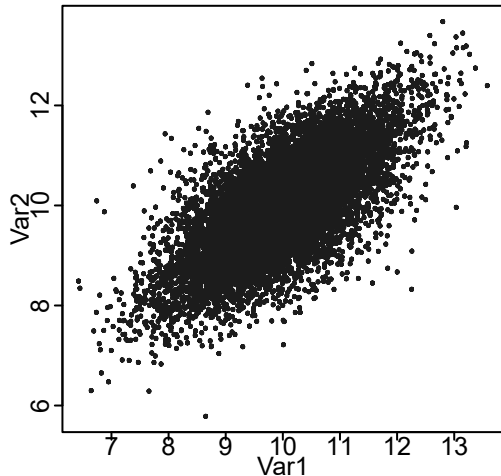
(a) Correlation = 0.7
