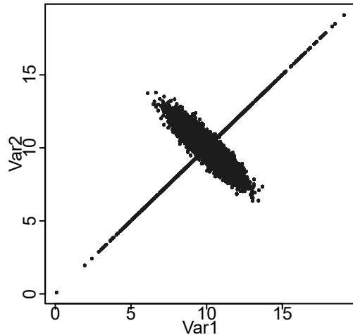
(b) Correlation = -0.05
