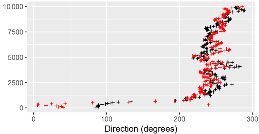
(c) Wind direction
