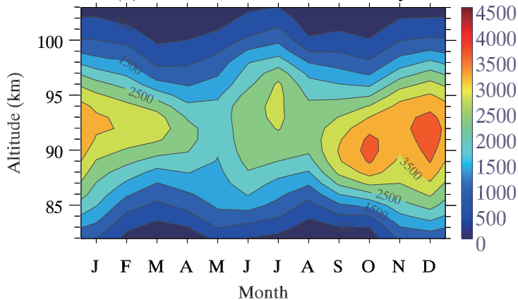
(a) USTC lidar sodium density
