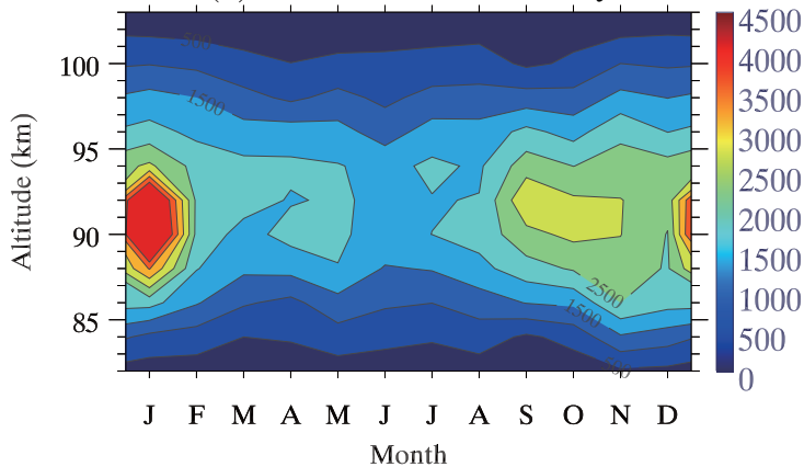
(b) OSIRIS sodium density
