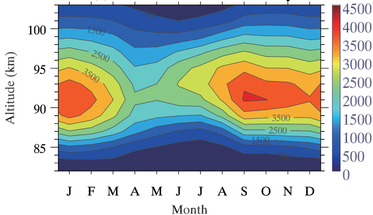
(c) WACCM sodium density
