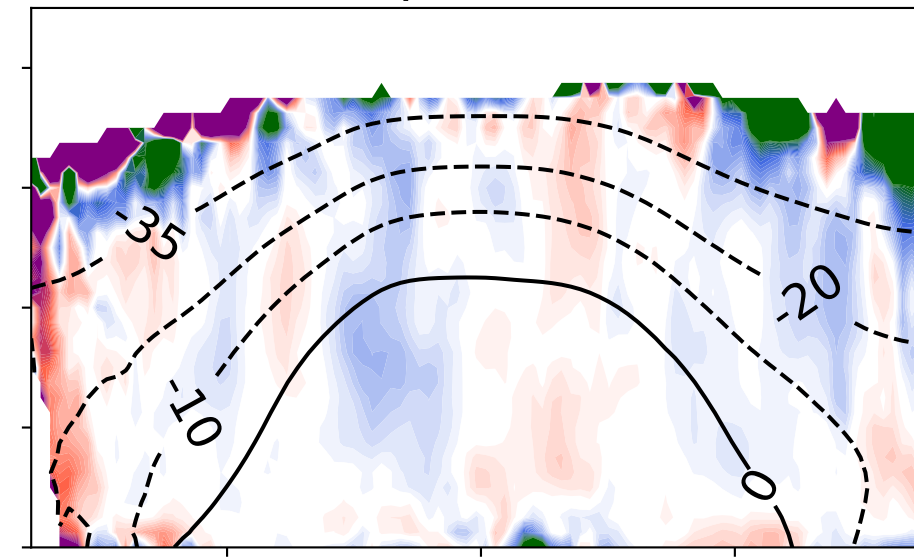
\Delta\text{cloud liquid occurrence}
