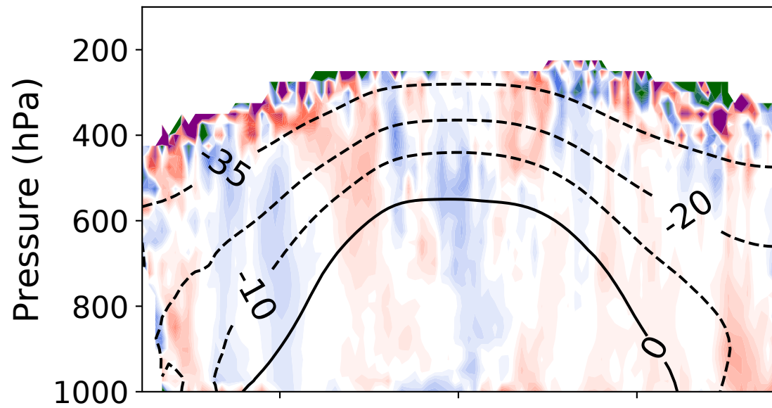
\Delta\text{CDNC}
