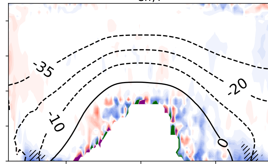
\Delta r_{\text{eff},i}
