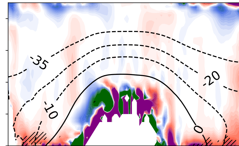
\Delta\text{cloud ice occurrence}
