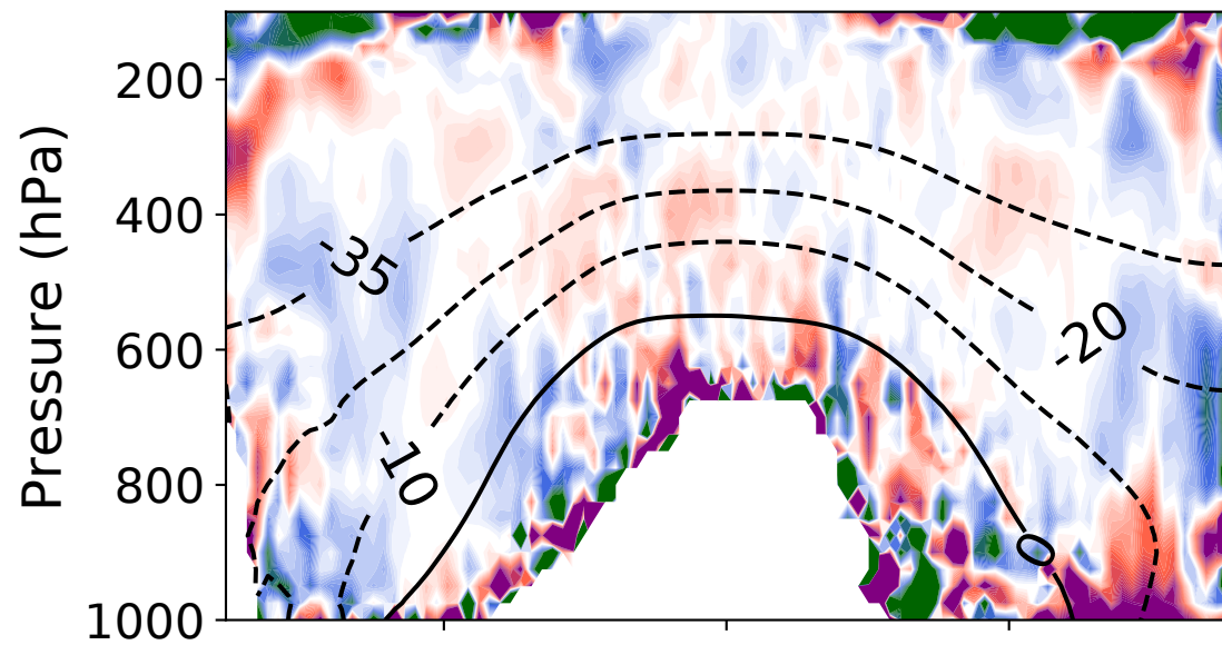
\Delta\text{ICNC}
