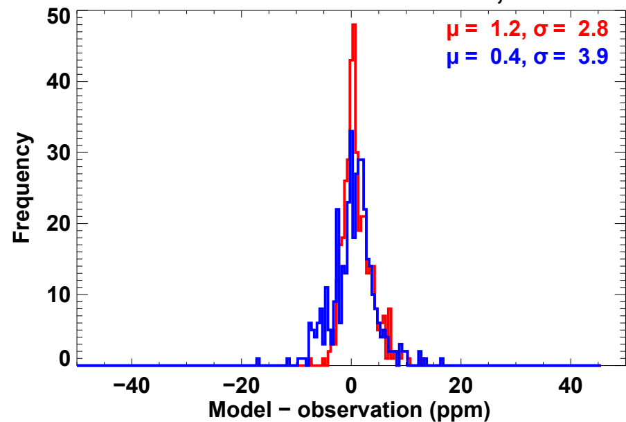
Model – AMAZONICA observations, above 2 km
