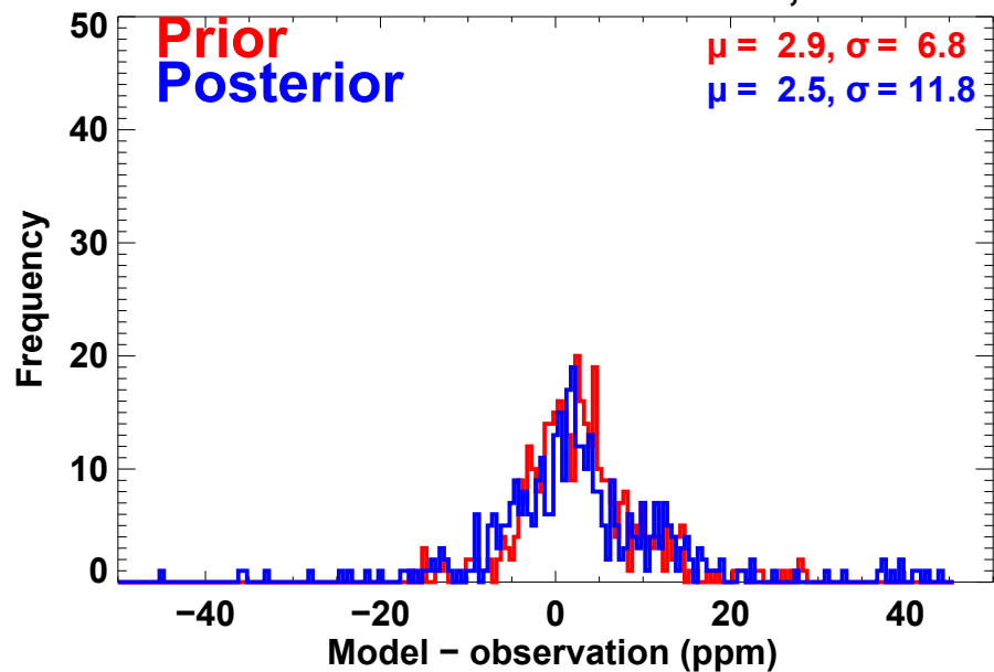
Model – AMAZONICA observations, below 2 km
