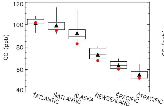
(c) MOPITT CO at 700 hPa
