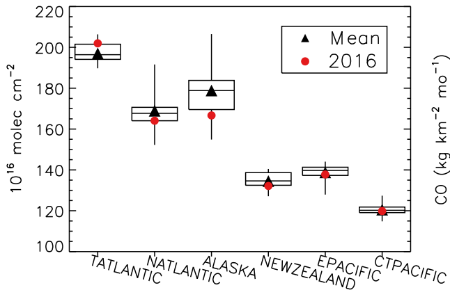
(a) MOPITT CO column
