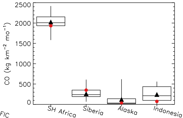
(b) GFED4 CO emissions
