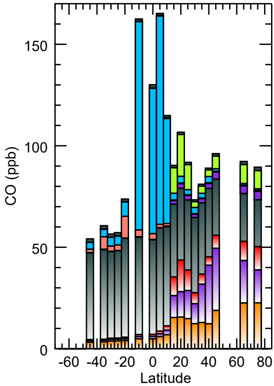
(b) Atlantic lower troposphere
