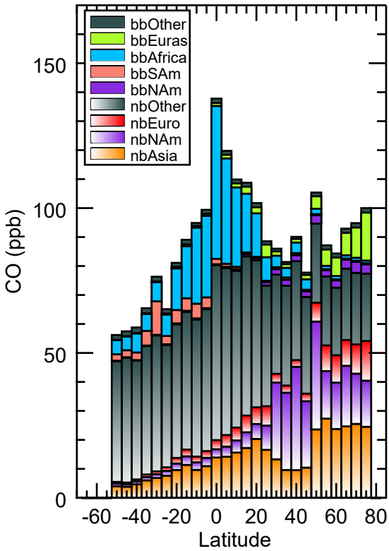
(a) Atlantic upper and middle troposphere
