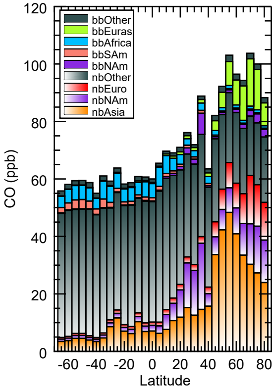
(a) Pacific upper and middle troposphere
