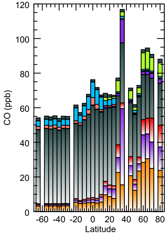
(b) Pacific lower troposphere
