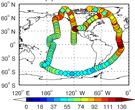
(b) GEOS-5 CO
