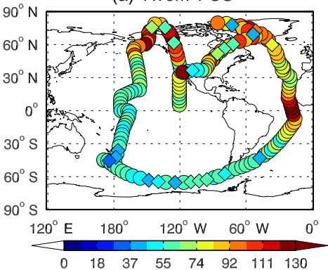
(a) ATom-1 CO
