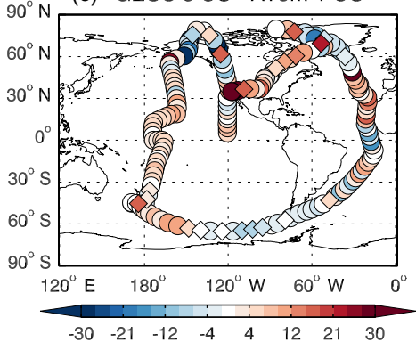
(c) GEOS-5 CO - ATom-1 CO
