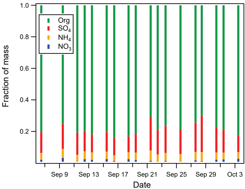
(c) Season-averaged particulate fractional composition
