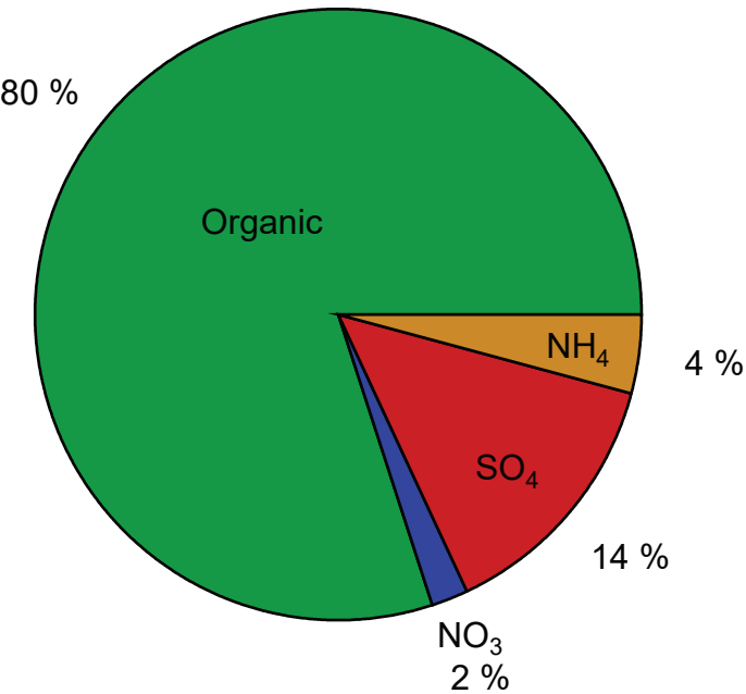
(c) Season-averaged particulate fractional composition
