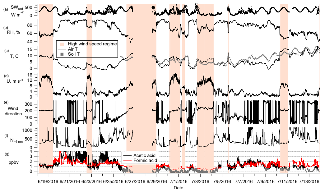
Figure 3. Time series of all data collected for the campaign (5 min averages). From top to bottom: total downwelling shortwave radiation, relative humidity, air temperature and soil temperature, wind speed, wind direction, aerosol particles, and FA (red) and AA (black, with values below the detection limit shown in gray.) The vertical axis is truncated at 4 ppbv for the organic acids and 1200\text{ cm}^{-3} for the aerosol particles. Orange bars highlight the high wind speed regime.
