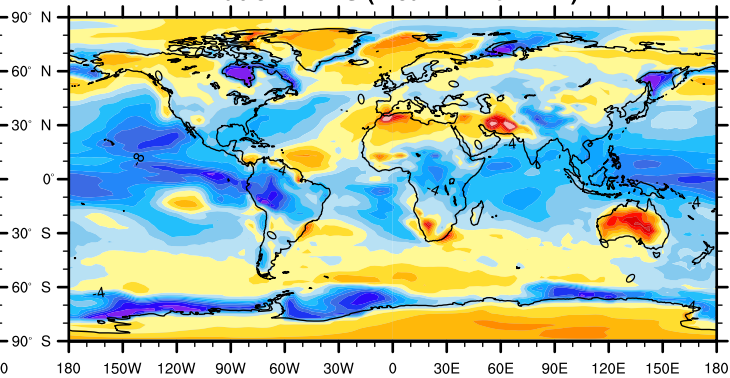
NorESM1-M (mean: -2.43 \text{ Wm}^{-2} )
