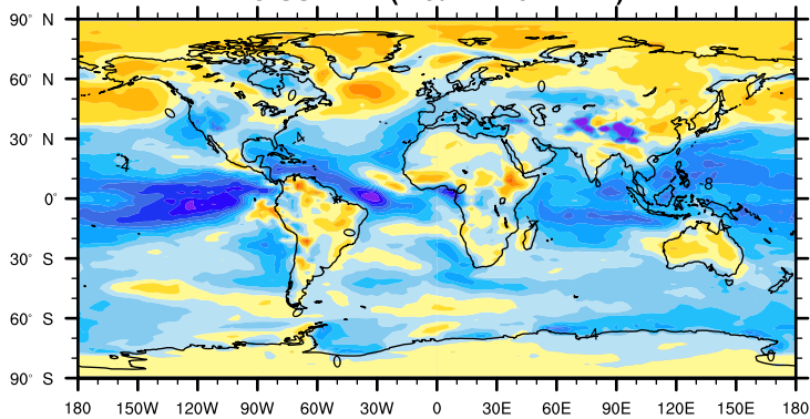
MIROC-ESM (mean: -3.40 \text{ Wm}^{-2} )
