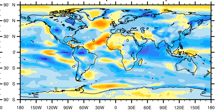
NorESM1-M (mean: -2.43 \text{ Wm}^{-2} )
