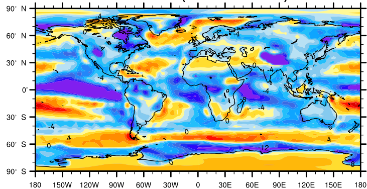
MIROC-ESM (mean: -3.40 \text{ Wm}^{-2} )
