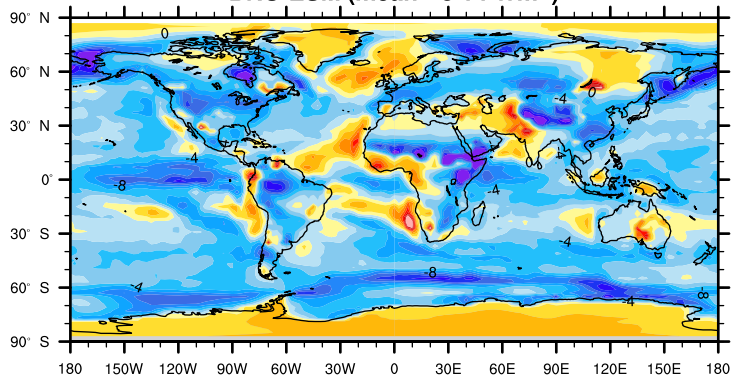
GISS-E2-R (mean: -2.67 \text{ Wm}^{-2} )
