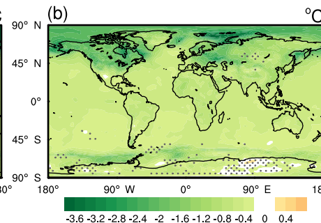
G4-rcp45
