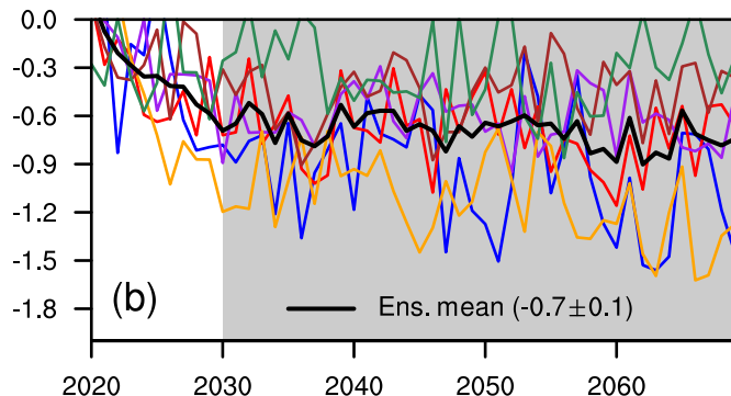
G4-rcp45
