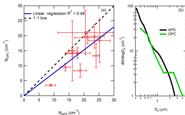
Figure 2. OPC concentrations with particle diameters ( D_p ) greater than 0.3\mu\text{m} (a) from 11 UAV research flights, listed in Table 1, plotted against APS concentrations ( D_p > 0.3\mu\text{m} ) at Mace Head Atmospheric Research Station (red circles). Error bars represent \pm 1 standard deviation. The points are fit with a linear regression (blue line). OPC data were averaged between 40 and 80 m a.s.l. OPC and APS number size distributions averaged for the 11 flights (b).
