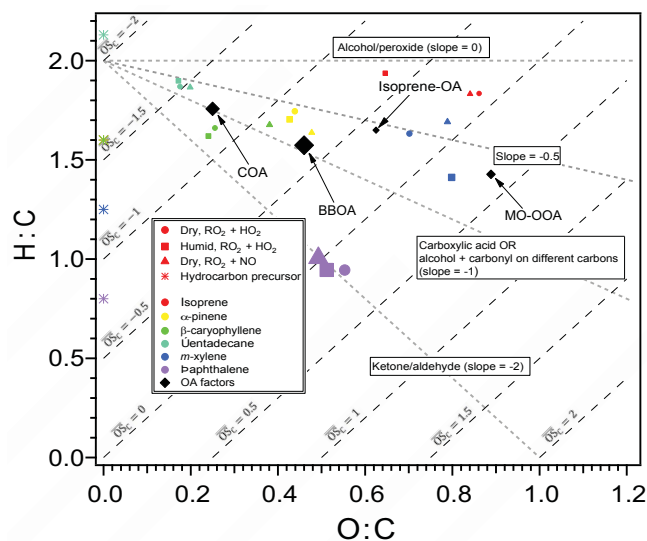
Figure 3. Van Krevelen plot for various SOA systems. Data points are colored by SOA system (red: isoprene, yellow: \alpha -pinene, green: \beta -caryophyllene, light blue: pentadecane, blue: m -xylene, and purple: naphthalene), shaped according to reaction conditions (circle: dry, RO 2 + HO 2 ; square: humid, RO 2 + HO 2 ; and triangle: dry, RO 2 + NO), and sized by intrinsic DTT activity. OA factors resolved from PMF analysis of ambient AMS data are shown as black markers, also sized by intrinsic DTT activity. Hydrocarbon precursors are shown as stars, colored by SOA system. Specifics on site locations and factor resolution methods are described elsewhere. COA: cooking OA, BBOA: biomass burning OA, Isoprene-OA: isoprene-derived OA, MO-OOA: more-oxidized oxygenated OA (Verma et al., 2015a; Xu et al., 2015a, b).
