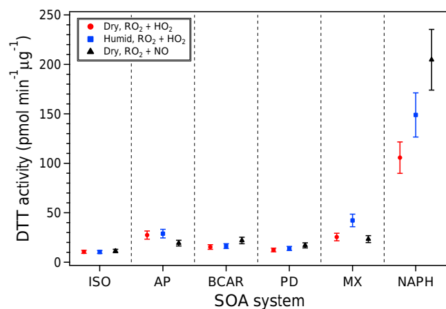
Figure 2. Intrinsic DTT activities for SOA generated from various hydrocarbon precursors (ISO: isoprene, AP: \alpha -pinene, BCAR: \beta -caryophyllene, PD: pentadecane, MX: m -xylene, and NAPH: naphthalene) under various conditions (red circles: dry, RO 2 + HO 2 ; blue squares: humid, RO 2 + HO 2 ; and black triangles: dry, RO 2 + NO). Dry RO 2 + HO 2 experiments were repeated to ensure reproducibility in SOA generation and collection. Error bars represent a 15% coefficient of variation (Fang et al., 2015b).
