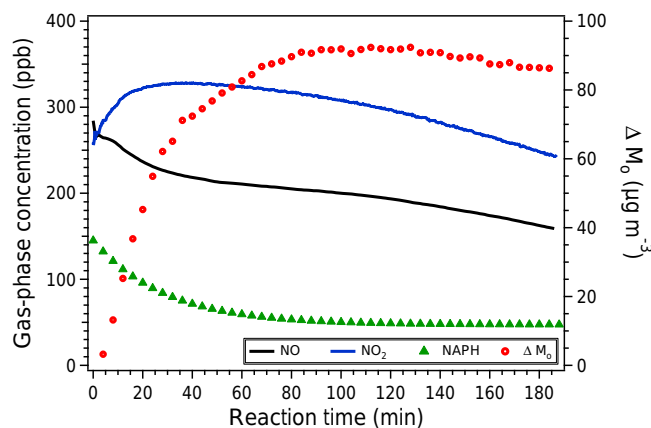
Figure 1. Typical reaction profile for a chamber experiment under \text{RO}_2 + \text{NO} -dominant conditions. NO and \text{NO}_2 concentrations were monitored by CAPS \text{NO}_2 and chemiluminescence \text{NO}_x monitors, respectively. Hydrocarbon decay was monitored using GC-FID, while initial hydrocarbon (naphthalene) concentrations were determined using the chamber volume and mass of hydrocarbon injected. Aerosol mass concentrations were determined using volume concentrations obtained from SMPS and assuming an aerosol density of 1 \text{ g cm}^{-3} . While typical SOA density is about 1.4 \text{ g cm}^{-3} , it varies with hydrocarbon precursor identity and reaction conditions, and a density between \sim 1.0 and 1.6 \text{ g cm}^{-3} has been reported in previous studies (Ng et al., 2006, 2007a, b; Chan et al., 2009; Tasoglou and Pandis, 2015; Bahreini et al., 2005). The use of a density of 1 \text{ g cm}^{-3} is to facilitate easier comparisons with past and future studies. Results from future studies can be scaled accordingly for comparison with the current work. Mass concentrations have been corrected for particle wall loss (Nah et al., 2016).
