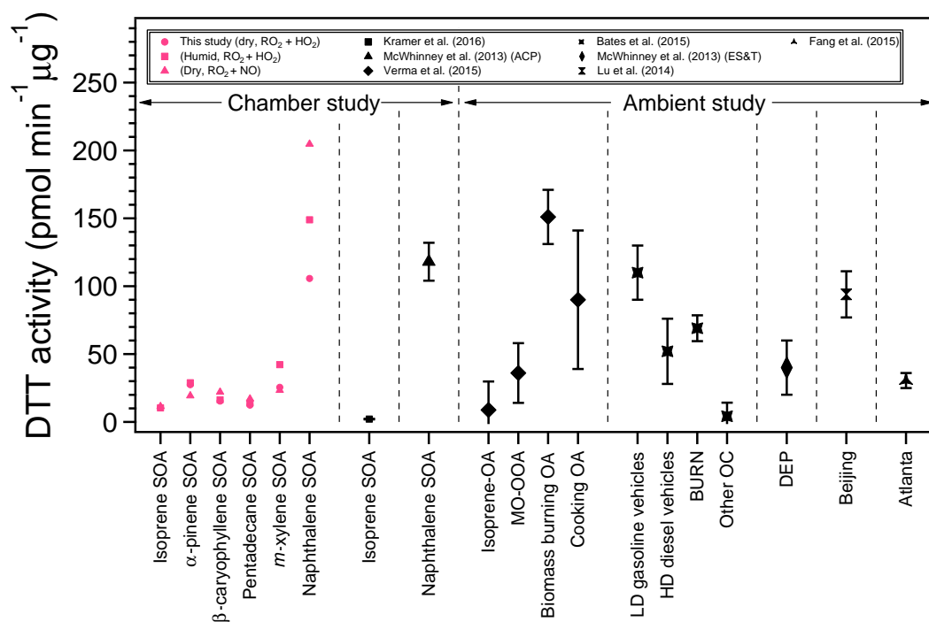
Figure 4. Intrinsic DTT activities for chamber SOA, various PM subtypes resolved from ambient data, and diesel exhaust particles. It should be noted that the DTT activity for isoprene SOA in Kramer et al. (2016) was determined using a different DTT method and may not be directly comparable. All other studies shown used the method outlined in Cho et al. (2005). DTT activities obtained in this study are shaped by reaction condition (circle: dry, \text{RO}_2 + \text{HO}_2 ; square: humid, \text{RO}_2 + \text{HO}_2 ; triangle: dry, \text{RO}_2 + \text{NO} ). Specifics on site locations and factor resolution methods are described elsewhere. DTT activities for Beijing and Atlanta are averages obtained across multiple seasons. Isoprene-OA: isoprene-derived OA, MO-OOA: more-oxidized oxygenated OA, BBOA: biomass burning OA, COA: cooking OA, LDGV: light-duty gasoline vehicles, HDDV: heavy-duty diesel vehicles, BURN: biomass burning, DEP: diesel exhaust particles (Kramer et al., 2016; McWhinney et al., 2013b; Verma et al., 2015a; Bates et al., 2015; McWhinney et al., 2013a; Xu et al., 2015a, b; Lu et al., 2014; Fang et al., 2015b).
