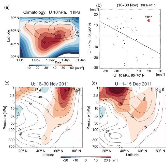
Figure 1. (a) Latitude–time section of the climatological zonal-mean zonal wind at 1 hPa (colour shading) and 10 hPa (contours). (b) Scatter diagram of the zonal-mean zonal wind averaged from 16 to 30 November over 25–35° N at 1 hPa (ordinate) and 60–70° N at 10 hPa (abscissa) for the period 1979–2015. The solid line indicates a regression line. (c) Height–latitude section of the zonal-mean zonal wind averaged from 16 to 30 November 2011. Contours and colour shading indicate the climatology and anomalies respectively. (d) Same as (c) but averaged from 1 to 15 December 2011.
