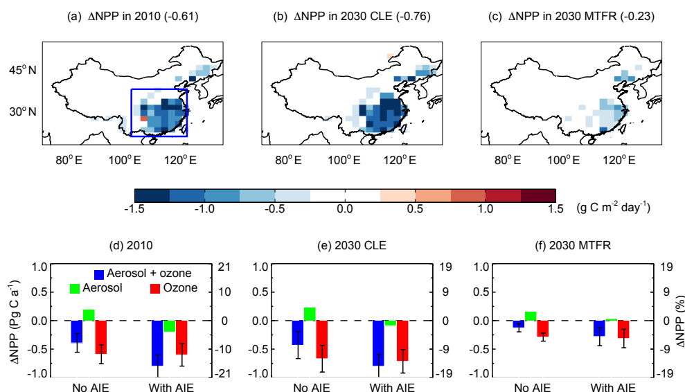
Figure 10. Impacts of air pollution on NPP in the whole of China. Results shown are combined effects of aerosol and O 3 on the summer NPP in (a) 2010, (b) 2030 with CLE scenario, and (c) 2030 with MTFR scenario. Results for the top panels do not include aerosol indirect effects (AIE) but do include the meteorological response to aerosol direct radiative effects. The average NPP perturbation over the box domain in panel (a) is shown in the bracket of each title. The perturbations to annual total NPP by aerosol, O 3 , and their sum over the whole China are shown in panels (d–f) for different periods, with (right) and without (left) inclusion of AIE. Damages by O 3 are averaged for low and high sensitivities with error bars indicating ranges. The percentage changes are calculated based on NPP without AIE. Simulations are performed with the ModelE2–YIBs model. Only the significant changes ( p < 0.05 ) are shown in panels (a–c).
