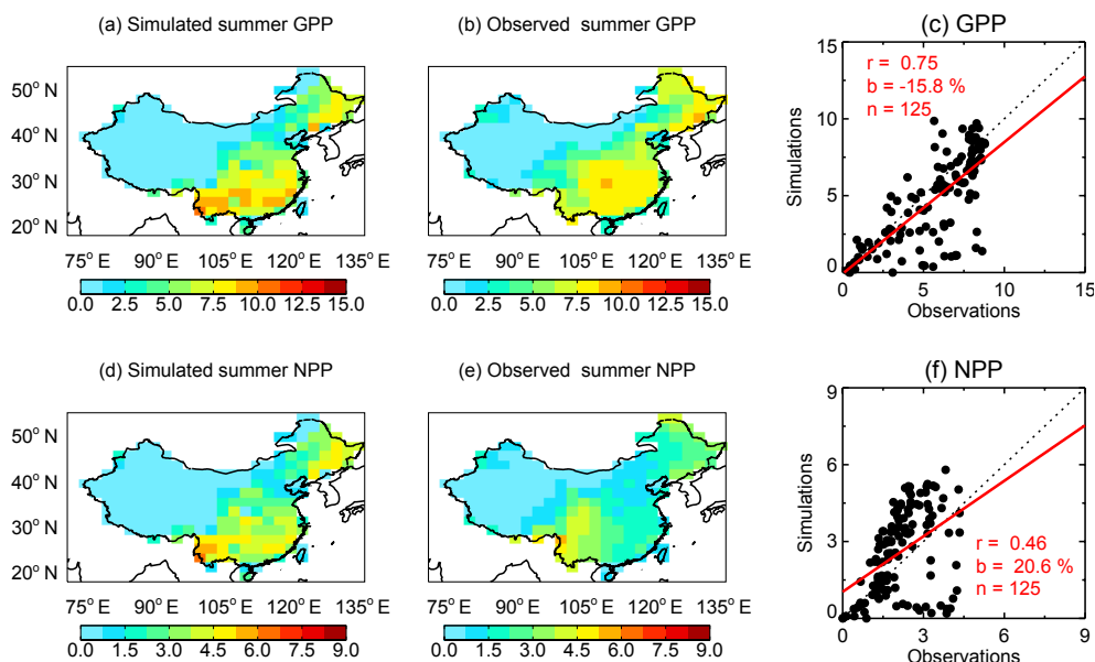
Figure 1. Evaluation of simulated summertime carbon fluxes by ModelE2-YIBs. Panels show GPP (top row) and NPP (bottom row) over China. Simulation results ( a , d ) are the average of G10ALLHO3 and G10ALLLO3, which are performed with the climate model ModelE2-YIBs using high and low ozone damage sensitivities (Table 2). The correlation coefficients ( r ), relative biases ( b ), and number of grid cells ( n ) for the comparisons are listed on the scatter plots. Units: \text{g C m}^{-2} \text{ day}^{-1} .
