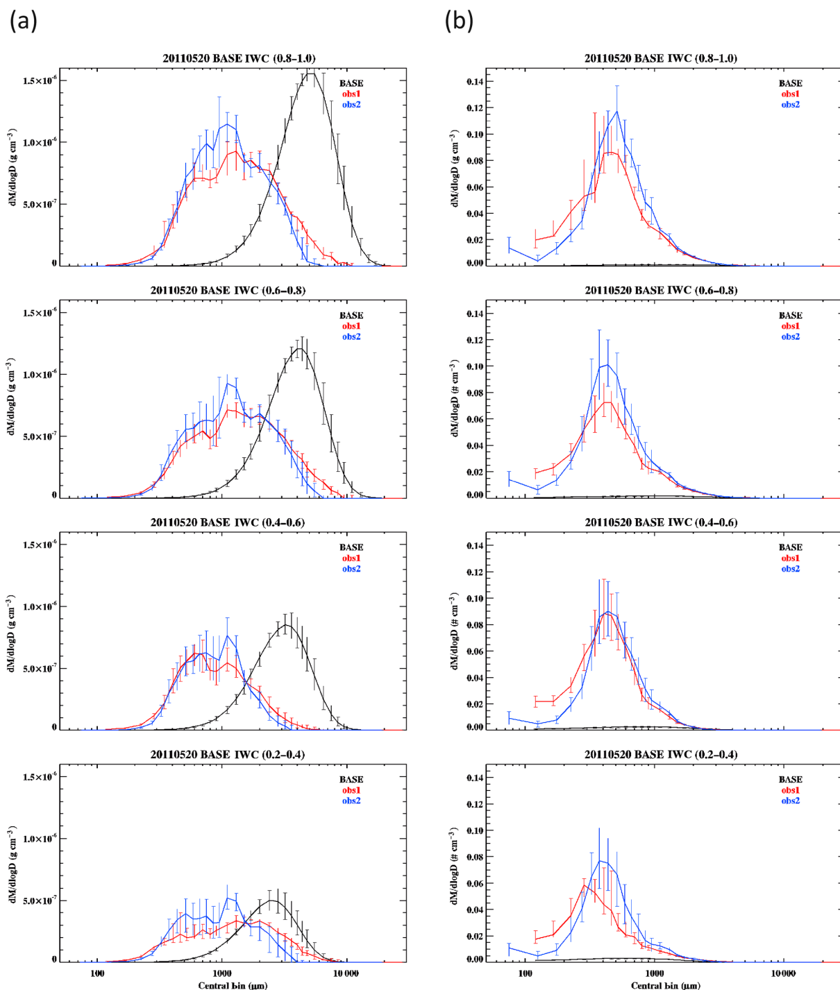
Figure 11. Size distributions of ice mass (a) and number (b) in four ranges of ice water content (IWC; ranges in parentheses in g m -3 ) derived from the merger of two-dimensional cloud (2DC) and high-volume precipitation spectrometer (HVPS) raw data independently by Wang et al. (2015a, “obs1” in red) and Wu and McFarquhar (2016, “obs2” in blue). Both are shown as an estimate of poorly established uncertainty. Also shown are size distributions from the BASE simulation (black) at 5.8 km (−11 °C) within the respective red-bounded geographic regions shown in Fig. 9. Simulated ice is the sum of all ice classes at each size. The simulated ice bin size is the sphere diameter calculated from the bulk density of each ice class. The measured ice size is the randomly oriented maximum dimension. Error bars indicate 1 standard deviation of values simulated or observed at each size.
