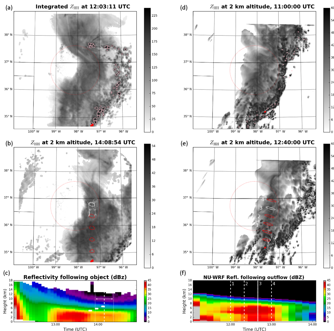
Figure 16. Horizontally polarized radar reflectivity ( Z_{HH} in dBZ) from KVN radar (dotted red circle): (a) example updraft object at \sim 12:00 UTC (solid red) among others identified in units of dBZ kilometers (red enclosed; see text); (b) movement of example updraft from initial location (solid red) towards intersection with the aircraft sampling location (white enclosed; see text) projected onto 2 km Z_{HH} at \sim 14:00 UTC; and (c) Z_{HH} curtain obtained from column-wise averages over tracked regions from \sim 12:00 to 15:00 UTC with Citation ascent legs in time and height (white bars) and averaging time used in Fig. 17 (white lines). From the AERO simulation: (d) identification of a typical updraft object projected onto simulated Z_{HH} at \sim 11:00 UTC (solid red) among others identified (red enclosed; see text); (e) its movement from the identified location (solid red) to the intersection with the aircraft sampling location (white enclosed; see text) projected onto simulated 2 km Z_{HH} at \sim 13:00 UTC; and (f) Z_{HH} curtain obtained from column-wise averages over tracked regions from \sim 11:00 to 14:00 UTC with the midpoint of hour-long averages used in Fig. 17 (white lines).
