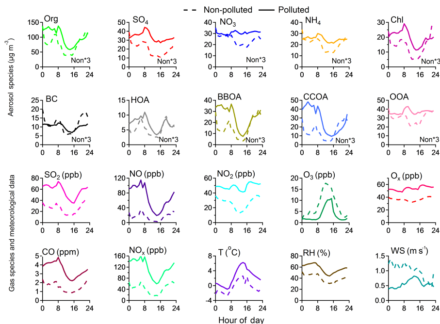
Figure 7. Average diurnal cycles of \text{PM}_{10} species, four OA factors identified via PMF analysis, various gas-phase species, and meteorological parameters on polluted and non-polluted days. The mass concentrations of aerosol species during non-polluted periods are scaled by three factors to highlight the differences in their diurnal trends on polluted and non-polluted days.
