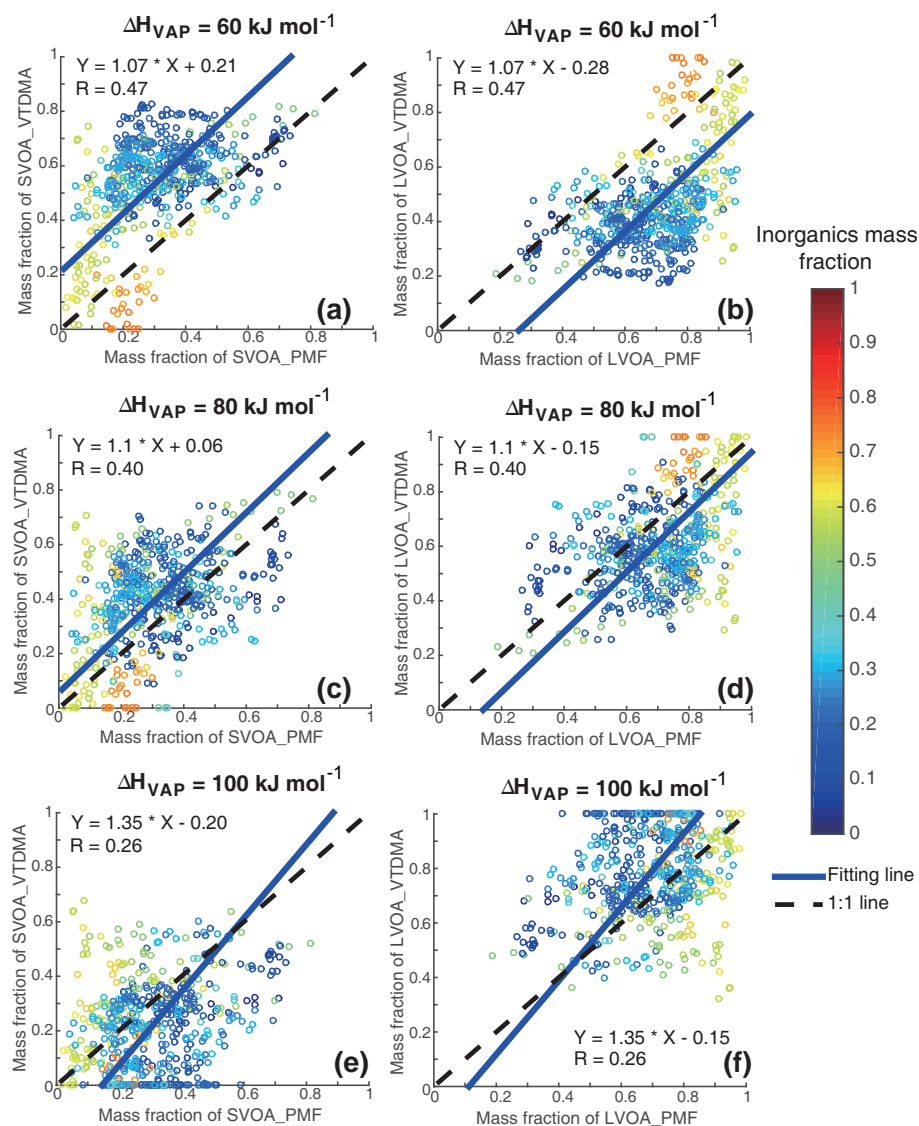
Figure 5. Mass fractions of SVOA and LVOA of the total organic mass obtained from VTMDMA data vs. the ones from the PMF analysis. Here, the y axis represents the VTMDMA results interpretation using the kinetic model and the x axis represents the AMS results interpretation using the statistical model (PMF). Model results were obtained by using a constant enthalpy value for all organics, corresponding to Combination 1 (a and b), Combination 2 (c and d) and Combination 3 (e and f) in Table 2. The LVOA_VTMDMA here is the sum of LVOA and ELVOA mass fractions. The colors of the data points illustrate the inorganic mass fraction in the particles. Correlation coefficient and equation for the line fitted to the data points are given in the legends.
