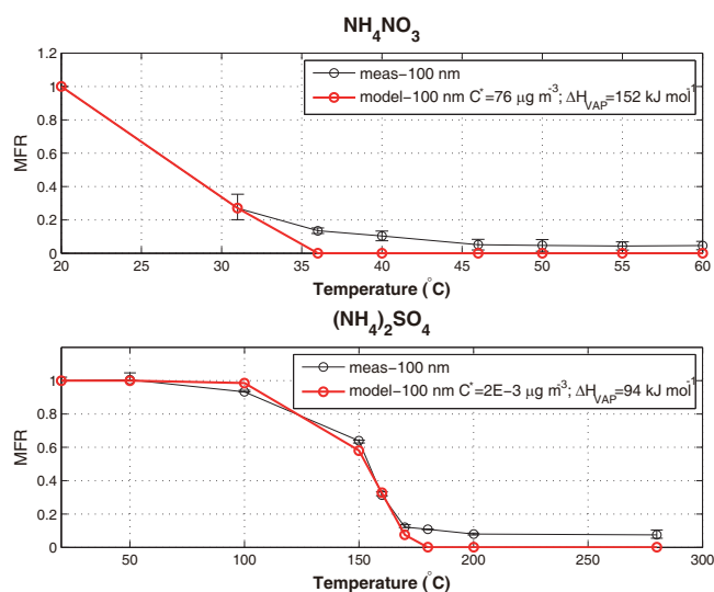
Figure 2. Thermograms of ammonium nitrate and ammonium sulfate using the VTDMA (black lines) and the modeled evaporation corresponding to the best fit with the experimental data (red lines).
