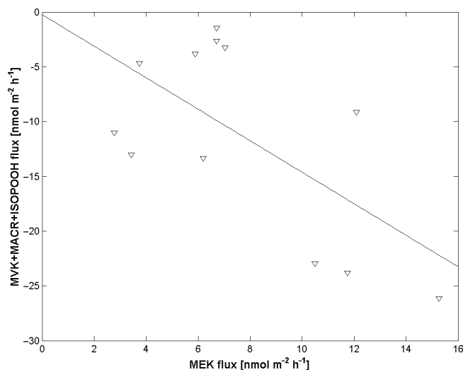
Figure 4. Scatter plot of branch-level MEK fluxes versus MACR + MVK + ISOPOOH fluxes during darkness in the period of 21–25 August. Linear fit parameters are the following: R^2 = 0.401 ; y = -1.44x - 0.24 .
