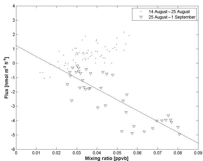
Figure 6. Flux measured as a function of mixing ratio for benzaldehyde during daytime of the whole branch-level measurement campaign. Black triangles represent the period of 25 August–1 September, when deposition dominated, and grey dots correspond to the period of 14–25 August, where mostly emission was measured. Linear fit parameters are the following: R^2 = 0.701 ; y = -75.59x + 1.22 .
