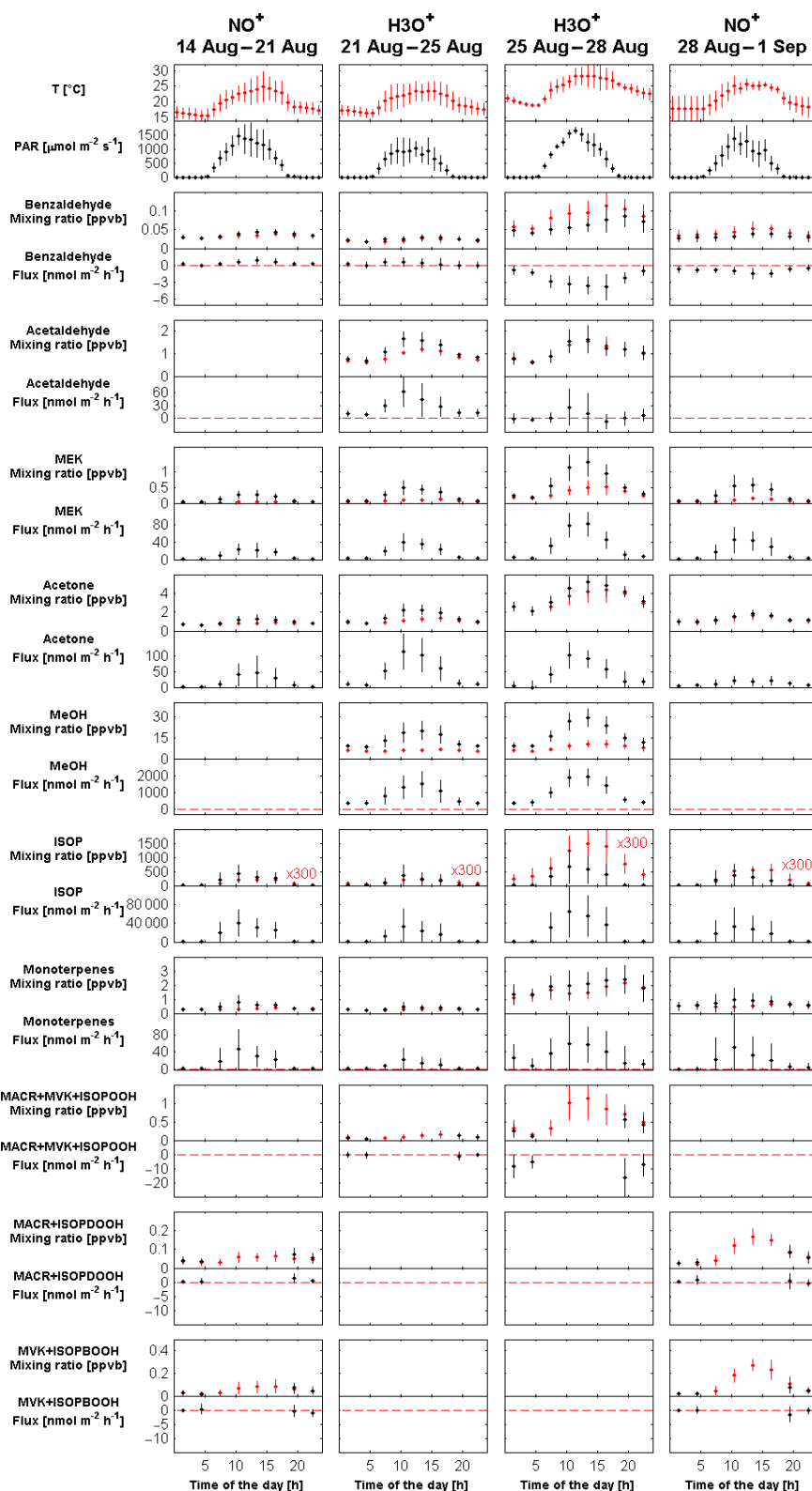
Figure 1. Diel average measured mixing ratios and fluxes in enclosures containing upper-canopy red oak branches at Harvard Forest. Mixing ratios of the inflow ambient air and of the outflow air are shown in red and black, respectively. Diel average temperature and PAR during the measurement period are also shown. Error bars represent standard errors of the data points in each time interval.
