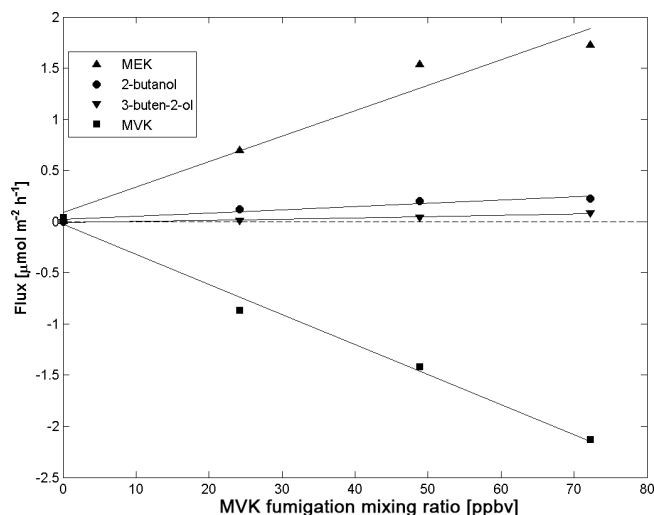
Figure 3. Example of branch-level VOC flux measured as a function of MVK fumigation mixing ratio during daytime. The concomitant MVK uptake and emission of MVK reduction products (namely MEK, 3-buten-2-ol, and 2-butanol) implies plant detoxification of MVK. Linear fit parameters are the following: MEK ( R^2 = 0.954 ; y = 0.0249x + 0.0869 ); 2-butanol ( R^2 = 0.928 ; y = 0.0031x + 0.0226 ); 3-buten-2-ol ( R^2 = 0.956 ; y = 0.0102x - 0.0102 ); MVK ( R^2 = 0.991 ; y = -0.0293x - 0.0279 ).
