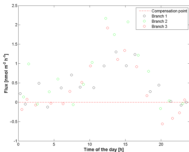
Figure 5. Example of benzaldehyde daily pattern for a day when benzaldehyde emission was detected. Measurements correspond to three different red oak upper-canopy branches.
