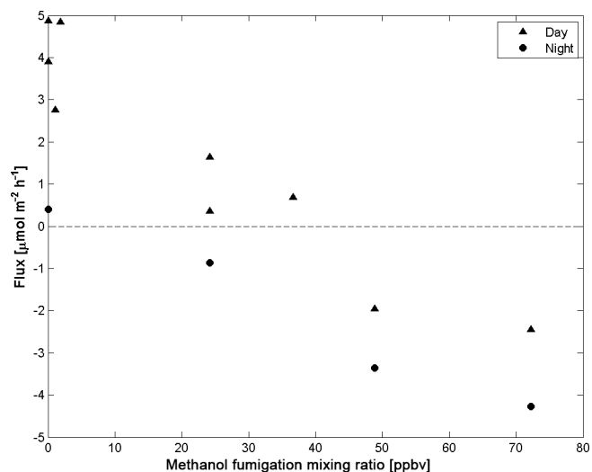
Figure 7. Example of enclosure flux measured as a function of fumigation mixing ratio for methanol in the field.
