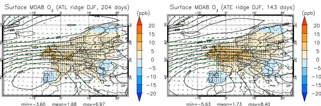
Figure 12. As Fig. 4 but for subtropical ridge centres in the Atlantic (30–0° W, left) and east Atlantic (15–0° W, right) in winter.
