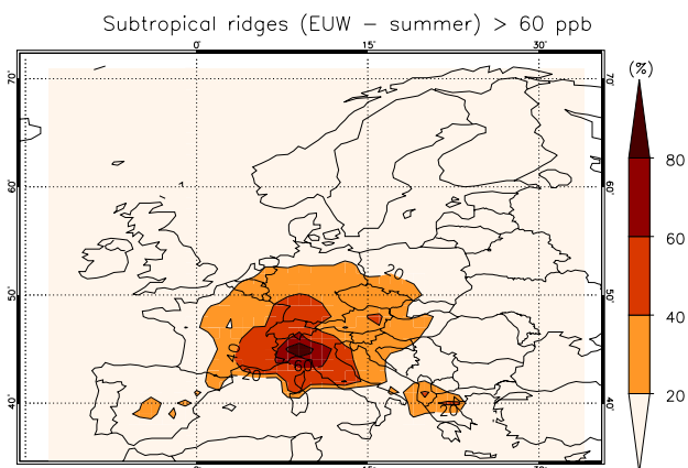
Figure 9. Percentage of summer days with ridge centres within the west flank of the EUR sector ( 0^{\circ} – 15^{\circ} E) for which the 60 ppb MDA8 O_3 target is breached. Note the similar geographic location of the region with exceedances on more than 40 % of the days in this figure and that where the local 90th percentile is surpassed on more than 30 % of the days under this synoptic situation (Fig. 7, upper right).
