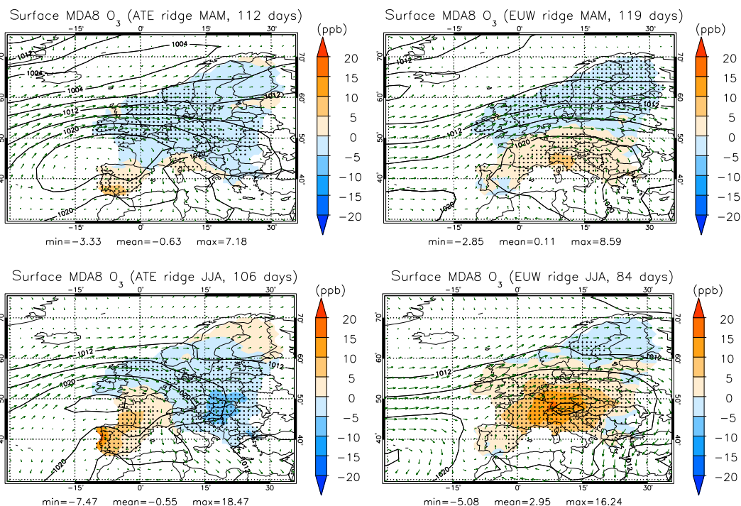
Figure 8. As Fig. 4 but for sub-tropical ridges with centres over the east Atlantic ( 15^{\circ} – 0^{\circ} W, left) and the west of the EUR sector ( 0^{\circ} – 15^{\circ} E, right) in spring (top) and summer (bottom).
