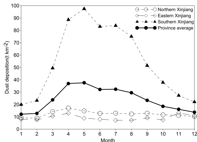
Figure 4. Monthly average dust deposition in Xinjiang Province from 2000 to 2013. Dust deposition in northern, eastern and southern Xinjiang is the average deposition at 8, 2 and 4 stations, respectively.
