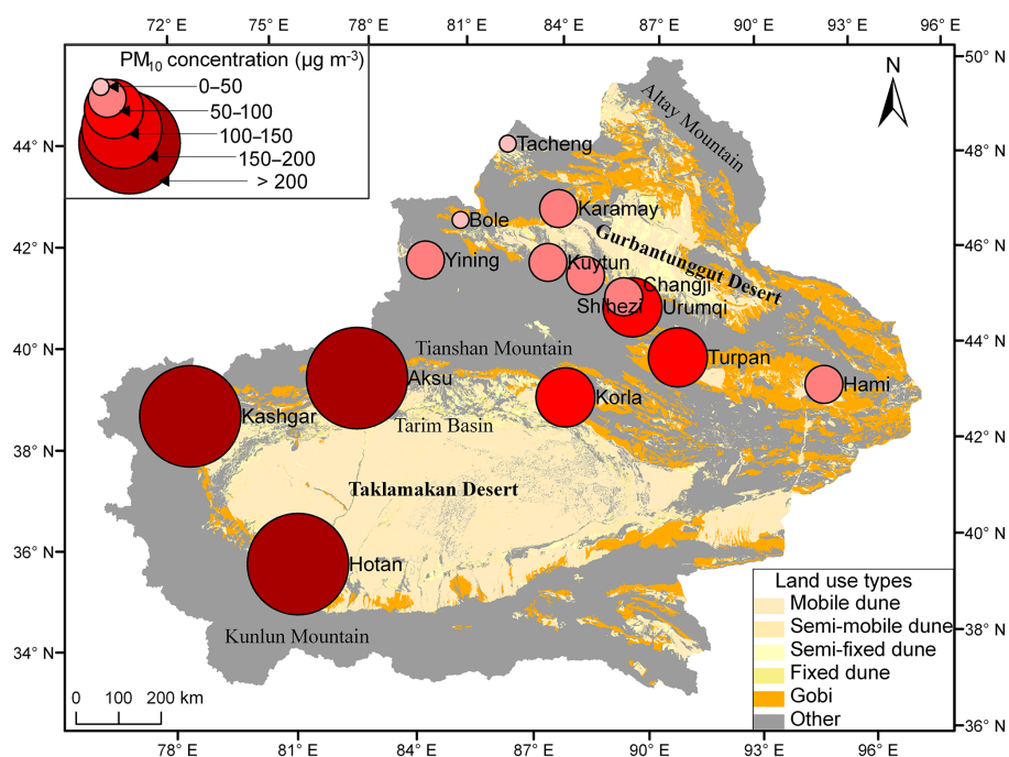
Figure 5. Annual average PM 10 concentration reported for 14 stations in Xinjiang Province from 2000 to 2013. Land use types are identified across the province according to Wang et al. (2005).
