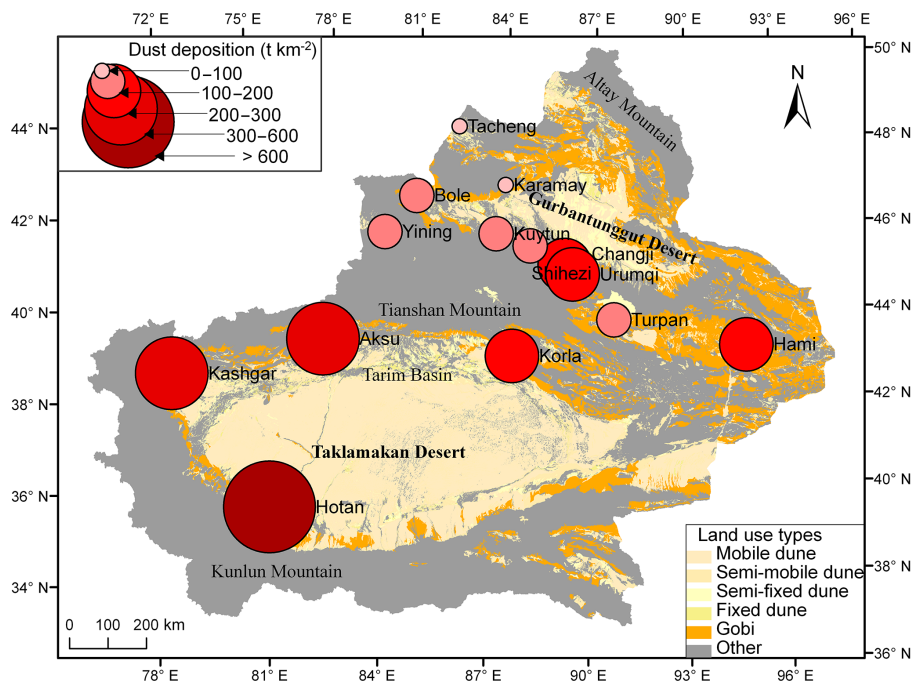
Figure 2. Annual average dust deposition reported at 14 stations in Xinjiang Province from 2000 to 2013. Land use types across the province are identified according to Wang et al. (2005).
