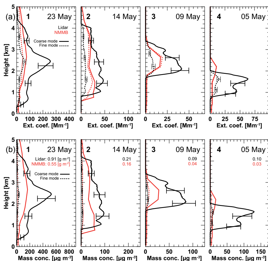
Figure 7. (a) Comparison fine (dotted) and coarse (solid) dust extinction coefficients derived from lidar observations (black) and simulated with NMMB/BSC-Dust (red). (b) Respective fine (dotted) and coarse (solid) dust mass concentrations derived from the lidar measurements (black) and simulated with NMMB/BSC-Dust (red). Column-integrated total dust mass concentrations are given as numbers.
