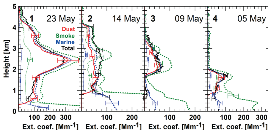
Figure 3. The Saharan aerosol layer as a function of distance from Africa (see Fig. 1, cases 1–4). Shown are the 532 nm particle extinction coefficients measured with Raman lidar (black curves) on 5–6 May, 23:40–00:35 UTC (case 4), 9 May, 23:15–24:00 UTC (case 3), 14–15 May, 23:45–00:20 UTC (case 2), and 23 May 2013, 03:45–05:00 UTC (case 1), and the extinction contributions by desert dust (red solid line) and marine (blue solid line, lidar ratio of 20 sr) or smoke and haze particles (green solid line, lidar ratio of 50 sr). The sums of dust and non-dust extinction contributions are given as thick dotted lines. If the black extinction curve is close to the blue dotted line, the non-dust aerosol component is probably of maritime origin (cases 1, 3, 4). In the case that the black and green dotted lines match, the non-dust aerosol component is most likely of anthropogenic origin (upper part of case 2).
