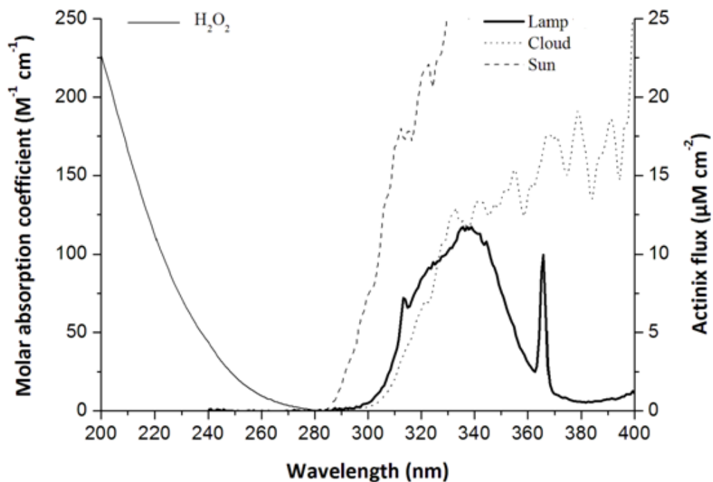
Figure SM1: Light spectrum of the lamp (Sylvania Reptistar) used for experiments compared to spectra of solar light measured on a sunny day and inside a cloud (measured on October 16, 2013 at 3:57-3:58 PM). Solar light and solar light inside a cloud were measured on the top of the puy de Dôme. H_2O_2 absorbance spectrum.
