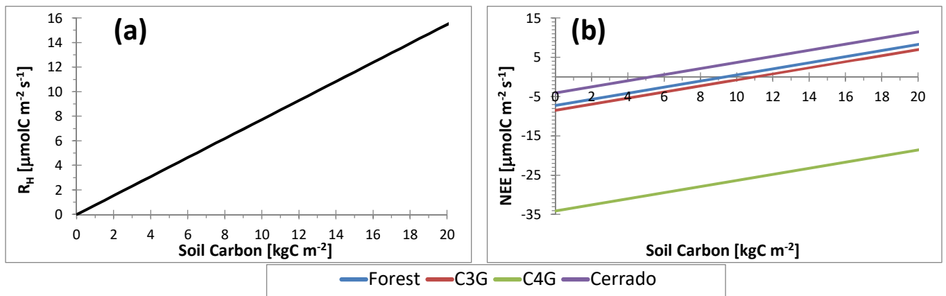
Figure S.2. Sensitivity test using JULES offline, running for a month (September 2010) and using the input data values shown in Figure S.1
