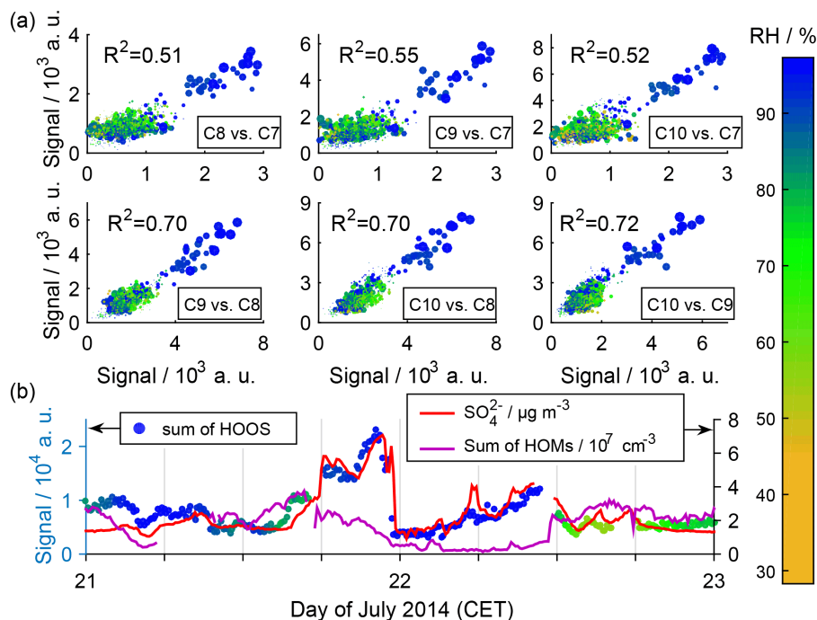
Figure 5. (a) Correlations among the selected HOOS signals as well as the effect of RH (color code) and particulate sulfate on their abundance (marker size, range: 0.8\text{--}7.2\ \mu\text{g m}^{-3} ). (b) Comparison of the sum of HOOS signals, particulate sulfate, and sum concentration of gas-phase HOMs during 21–23 July, demonstrating good agreement between HOOS and sulfate for high RH periods.
