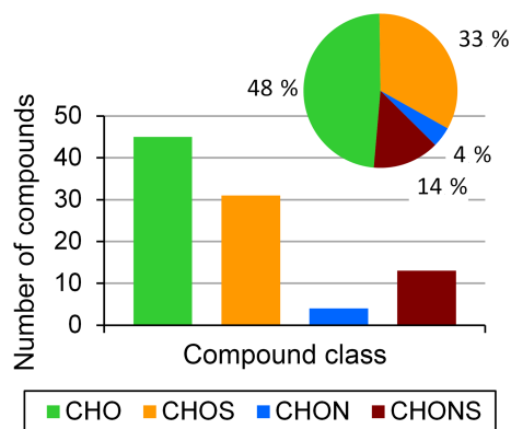
Figure 1. Number and fraction of identified compounds by LC-MS analysis of filter sample extracts for each compound class.
