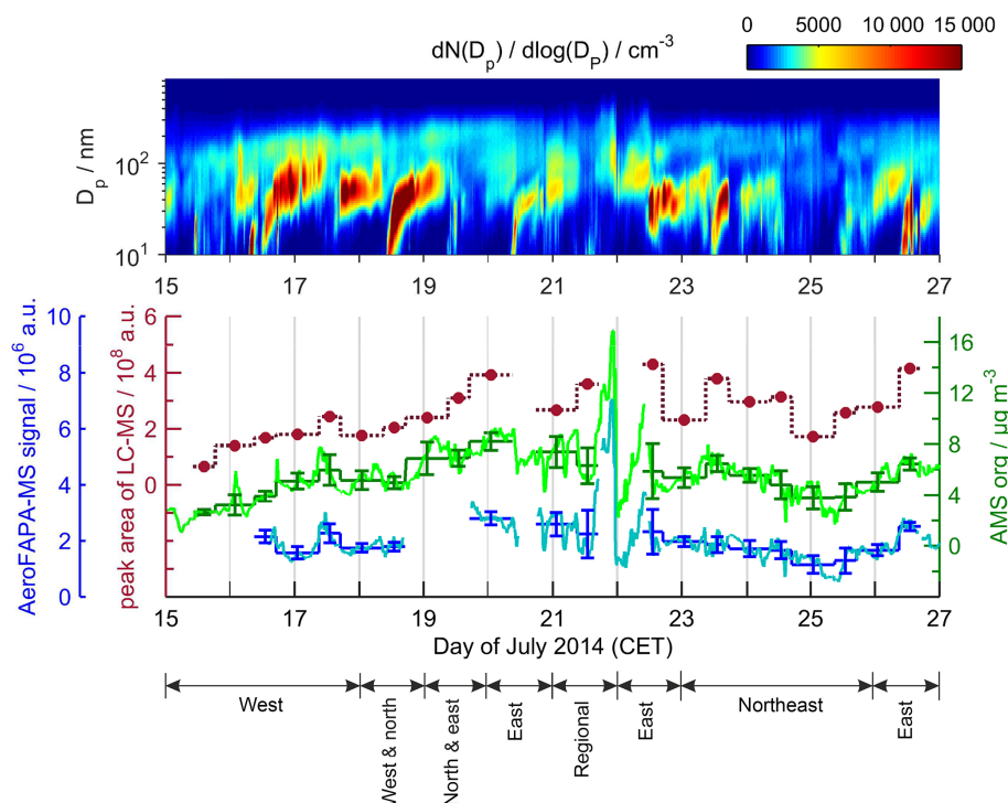
Figure 2. Top panel: number size distribution of aerosol particles, which was measured by the T-SMPS. Middle panel: sum of the peak areas for the 93 identified compounds from the filter samples by LC-HRMS (red). The signals for these compounds, measured by AeroFAPA-MS (blue), and the organic aerosol mass, measured by an AMS (green), show similar trends. Averaged values for the filter sampling times are depicted by the horizontal lines (error bars show 1 standard deviation). Bottom panel: major source directions of 96 h backward trajectories arriving at the site (250 m a.g.l.).
