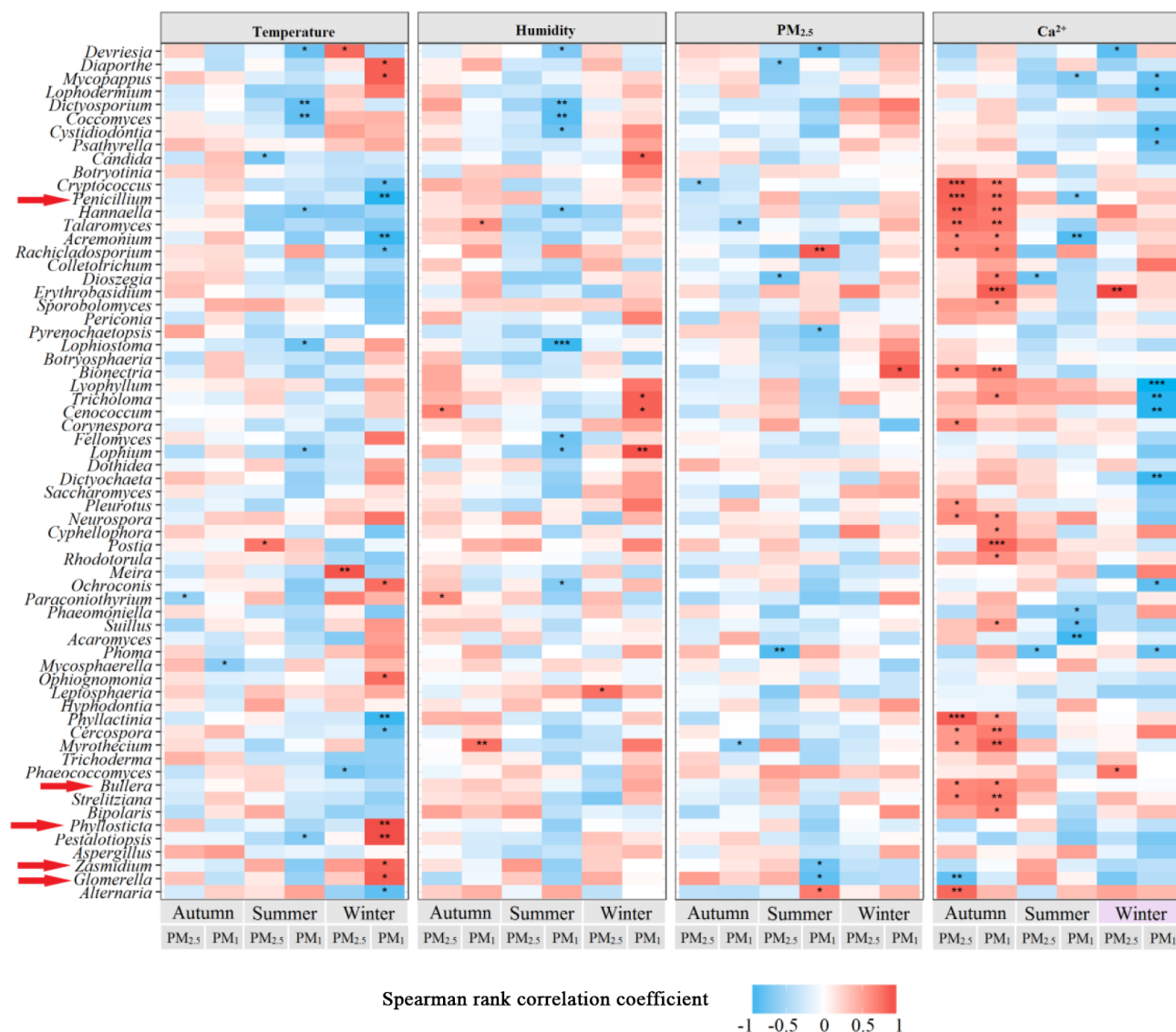
Figure 5. Heatmap analysis of the top 64 fungal genera based on Spearman's rank correlations (** p < 0.001 ; * p < 0.01 ; * p < 0.05 ). Red arrows indicate that the specific fungi varied significantly in different seasons.
