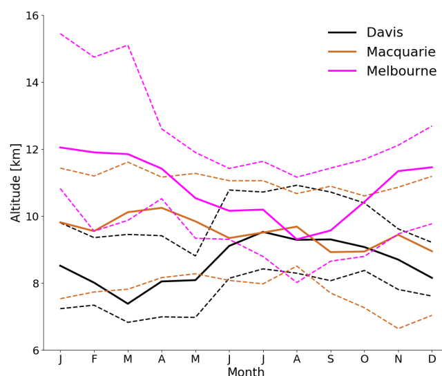
Figure 2. Multi-year monthly median tropopause altitude (using the ozone-defined tropopause) determined from ozonesondes measurements at Davis (2006–2013), Macquarie Island (2004–2013), and Melbourne (2004–2013) (solid lines). Dashed lines show the 10th to the 90th percentile of tropopause altitude for each site.
