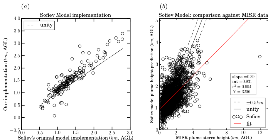
Figure 7. Comparison of our implementation of the plume rise parameterisation of Sofiev et al. (2012) to (a) the original results from Sofiev et al. (2012) for the same fires, and (b) plume stereo-height retrievals extracted from the North-American subset of the (MISR) plume height project data Nelson et al. (2008), derived using the MINX tool as shown in Fig. 4. Our implementation of the Sofiev et al. (2012) model differs from the original in its definition of the PBL height, which in our approach is extracted from the diagnostic product of ECMWF forecast runs (ECMWF, 2012). See Figs. 9 and 10 for a statistical overview of the Northern American MISR data set. Note that the Sofiev et al. (2012) model did not retrieve simulated plume heights for all the 3320 selected fires of that dataset. For 114 fires, either the Brunt-Vaisala frequency could not be retrieved or the FRP of the most powerful pixel listed in the MISR product were unavailable (see Sofiev et al., 2012, for details in the initialisation of the model).
