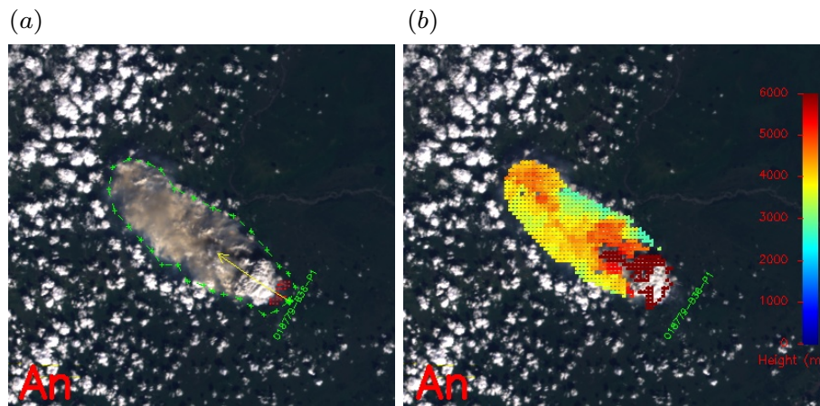
Figure 4. Example of smoke plume height derivation using data from the Multiangle Imaging SpectroRadiometer (MISR) that operates on the Terra satellite. The fire took place on the 29 June 2003 in Alaska, and was observed by MISR at 21:41 UTC and is referenced in the MISR data set as 018779-B36-P1. The user-defined smoke plume contour shown in (a) is used by the MINX software (Nelson et al., 2008) to derive the plume stereo-heights shown in (b). Background images are the MISR nadir views, and the locations of MODIS-derived active fire pixels are shown in red on (b). Image taken from the MISR plume height project website (see Footnote 1).
