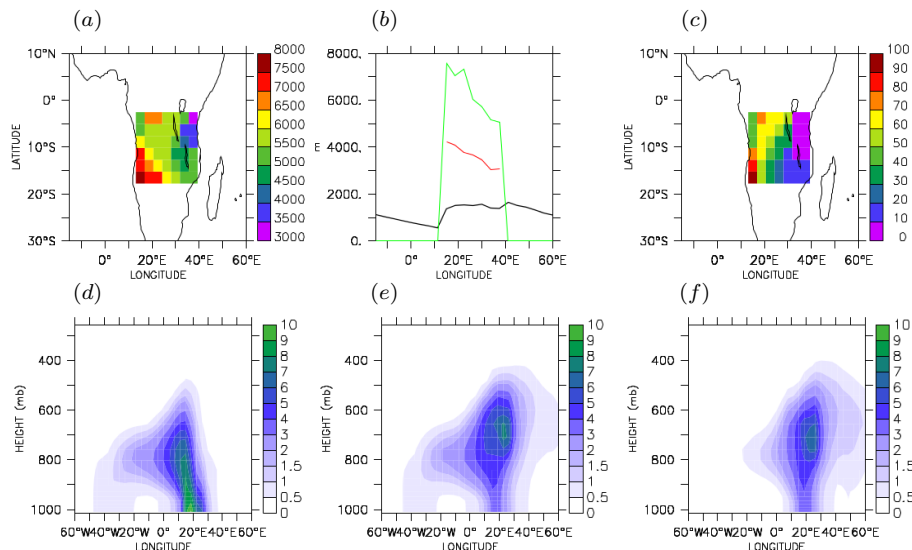
Figure 8. Simulations performed using the pyro-EDMF plume rise model of Rio et al. (2010) for sub-Saharan Africa between 10 and 30 July 2006. In the upper panel (a) shows the maximal injection height of CO 2 emissions simulated with the LMDZ model and pyro-EDMF between 5 and 20° S over the 20 days of the simulation. (b) reports the maximal injection height (green), mean injection height of emissions injected above the boundary layer height (red), and mean boundary layer height (black) averaged between 5 and 20° S altitude and over the 20 days of the simulation. (c) shows the percentage of cases for which the injection height passing the boundary layer height. In lower panel (e) shows the averaged vertical distribution of CO 2 mixing ratio (ppmv) for the same reference simulation and (d) for simulations without pyro-EDMF, and (f) with pyro-EDMF set up with a lower value of the ratio \beta = entrainment/detrainment = 0.1 (right). The reference simulation in (e) uses a value of \beta = 0.4 . Figure from Rio et al. (2010).
