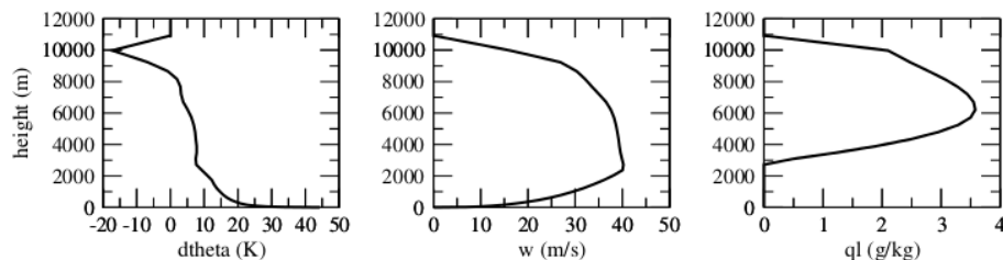
Figure 6. Smoke plume characteristics for the Chisholm fire, as simulated by pyro-EDMF: virtual potential temperature (K), vertical velocity excess ( \text{m s}^{-1} ), and cloud liquid water ( \text{g kg}^{-1} ) are shown. Figure from Rio et al. (2010).
