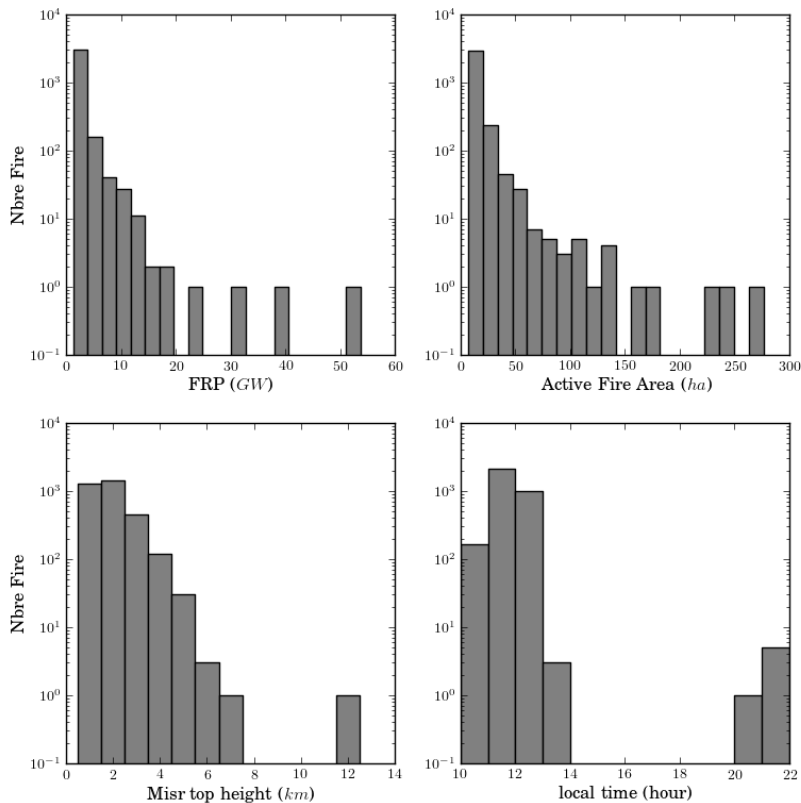
Figure 10. Distribution of FRP, Active fire Area, top plume height, and local time observation time for the 3320 fires of the current North American subset of the Multi-angle Imaging Spectro Radiometer (MISR) plume height project dataset Nelson et al. (2008) derived using the MINX tool shown in Fig. 4.
