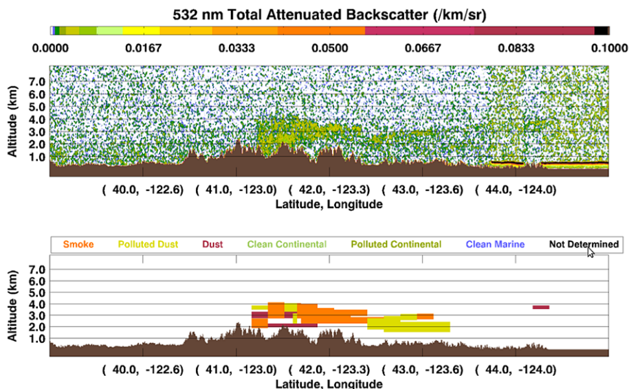
Figure 3. Example of profiles for Level-1 CALIOP 532 nm total attenuated backscatter data product (top), and the matching level-2 product of aerosol layers (bottom) for the 28 August 2006 over the Klamath mountains in California and Oregon. The presence of aerosols classified as biomass burning smoke can be seen. Image from Raffuse et al. (2012).
