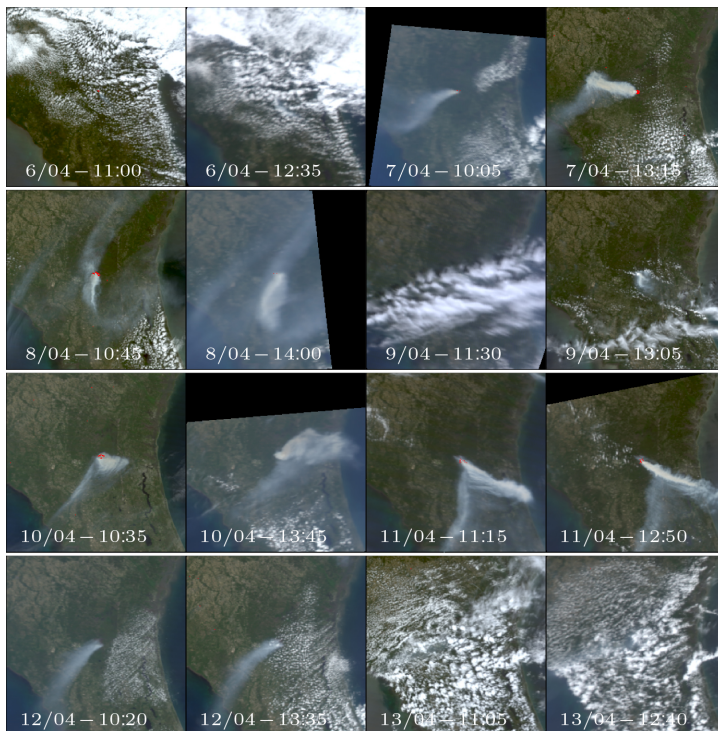
Figure 1. True colour composite of daytime observations of the County fire (US), made from the Moderate Resolution Imaging Spectroradiometer (MODIS) satellite EO sensor. The fire occurred in Ocala National Forest (Florida) between 5 and 13 April 2012. MODIS data from all available Terra and Aqua satellite overpasses are shown, with the local time indicated. Overlain on the colour composite imagery are red vectors that outline pixels detected as containing active fires by the MODIS MOD14/MYD14 Active Fire and Thermal Anomaly Products (Giglio et al., 2003). The regularly changing nature of the fire and the smoke transport apparent from this time series, as well as the presence on some days of bifurcated plumes, is very apparent.
