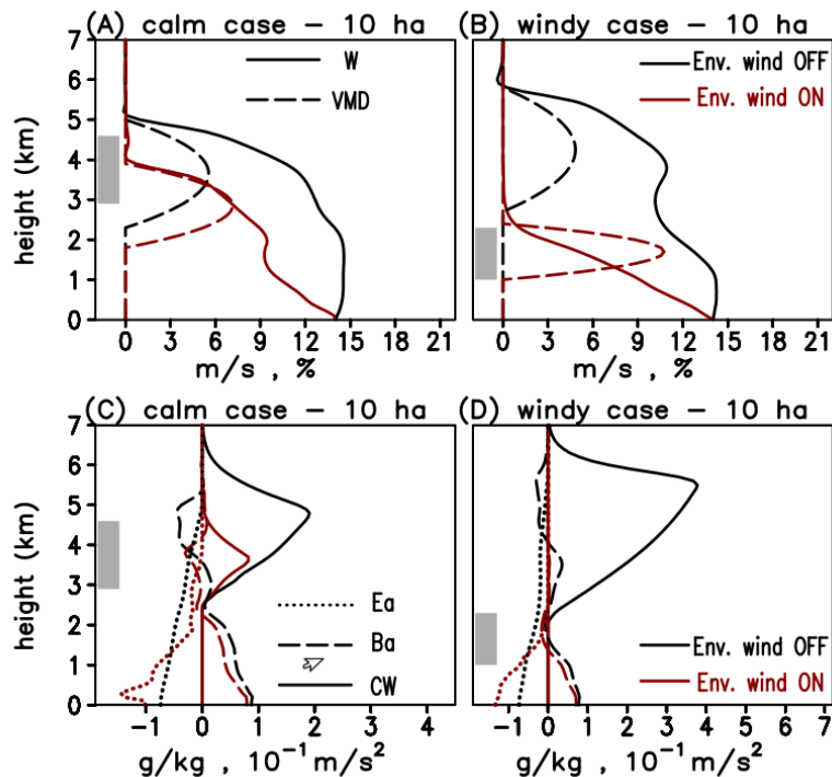
Figure 5. Results from the 1-D plume rise model (PRM) of Freitas et al. (2007, 2010) for a fire burning in (a, c) calm and (b, d) windy atmosphere scenario, as studied by Freitas et al. (2010). The fire has an active fire area (AF-area) of 10 ha. The quantities shown are: vertical velocity ( W , \text{m s}^{-1} ), vertical mass distribution (VMD, %), entrainment acceleration ( E_a , 10^{-1} \text{ m s}^{-2} ), buoyancy acceleration ( B_a , 10^{-1} \text{ m s}^{-2} ), and total condensate water (CW, \text{g kg}^{-1} ). Model results considering the environmental wind drag are shown in red, whilst those in black depicts the results from simulations disregarding this effect. Grey rectangles indicate the main injection height simulated by the 3-D ATHAM model (Trentmann et al., 2006) for the same fire scenario. Figure from Freitas et al. (2010).
